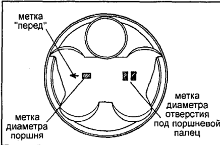
4A-GE.
