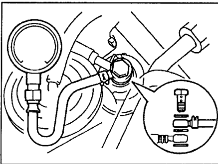
4A-GE.
