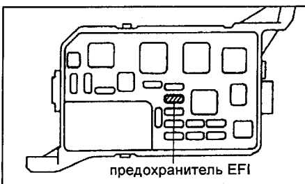
4A-GE.
