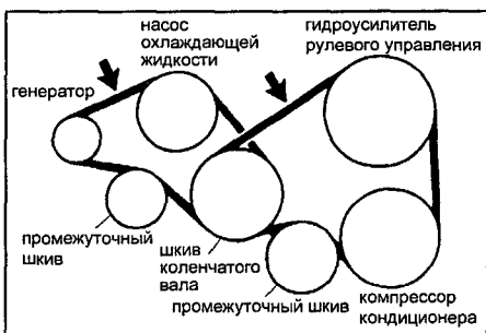
4A-GE.
