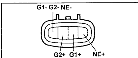
4A-GE.
