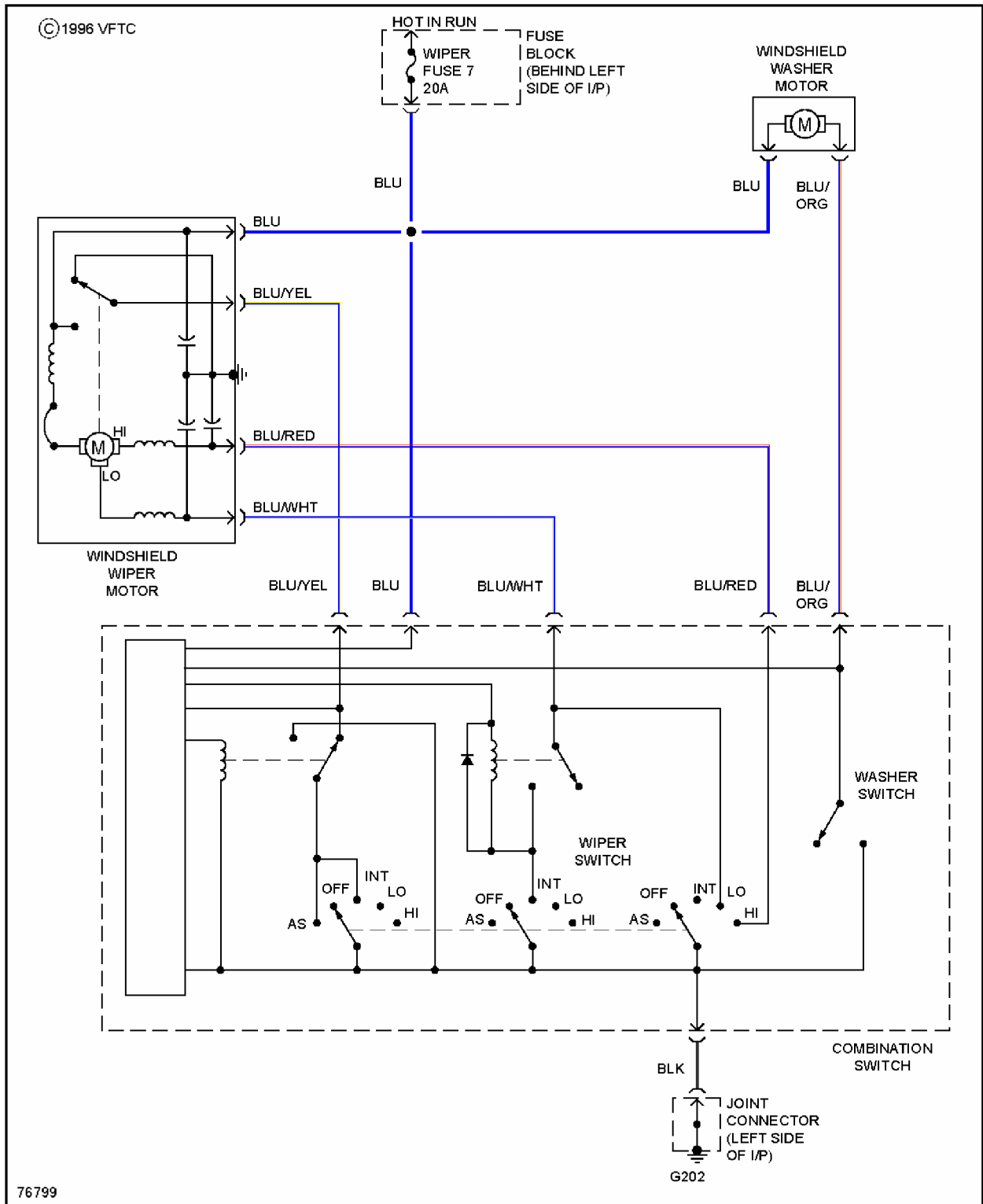
Fig. 7: Wiper/Washer Circuit, Canada
