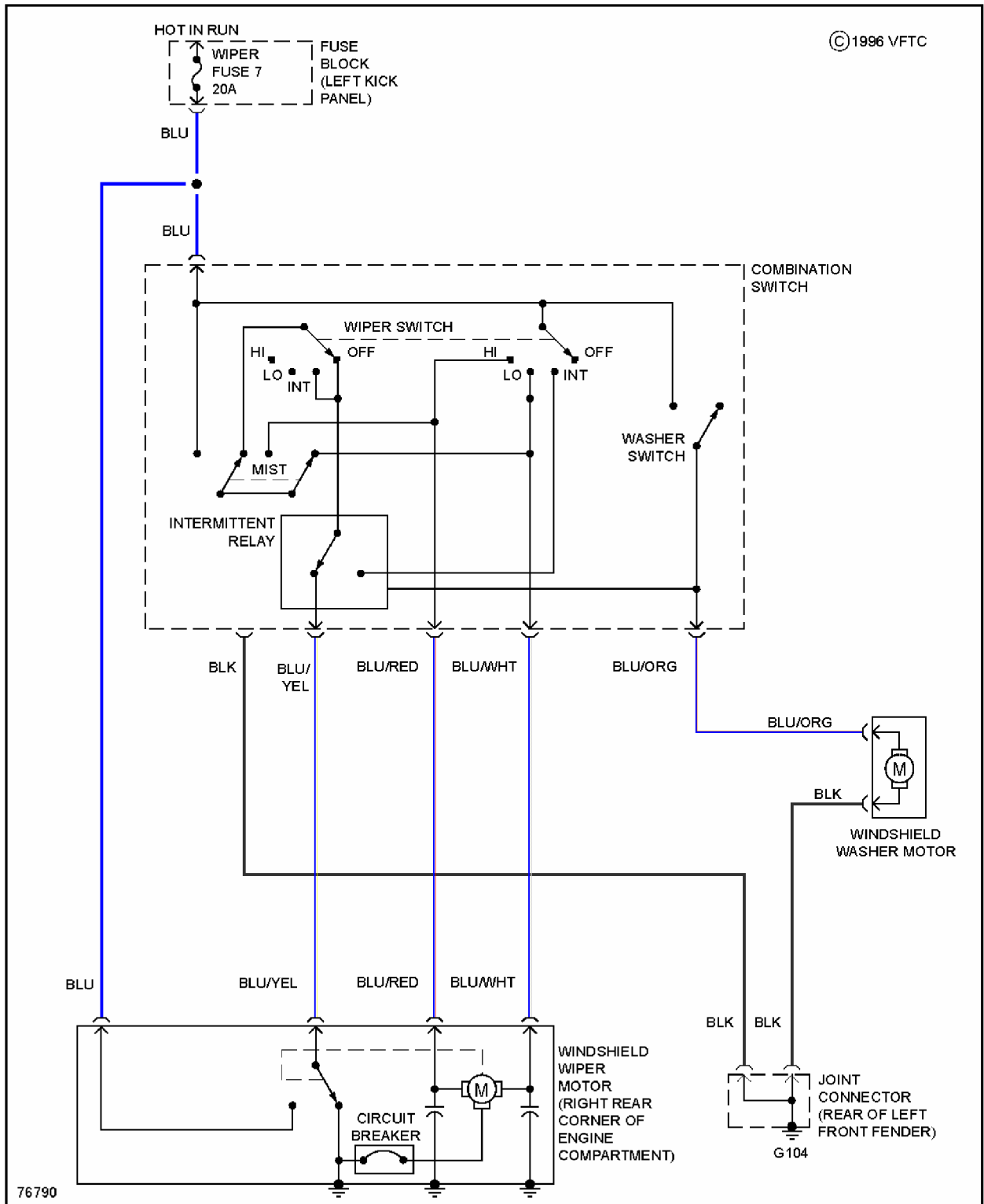
Fig. 8: Wiper/Washer Circuit, USA
