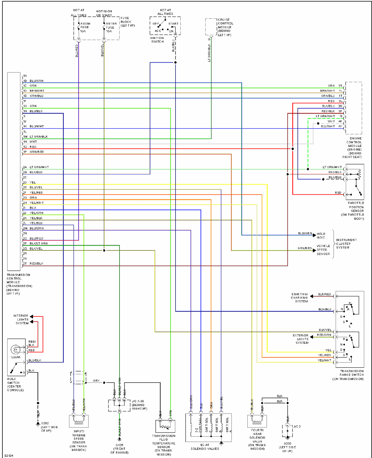
Fig. 30: Transmission Circuit
