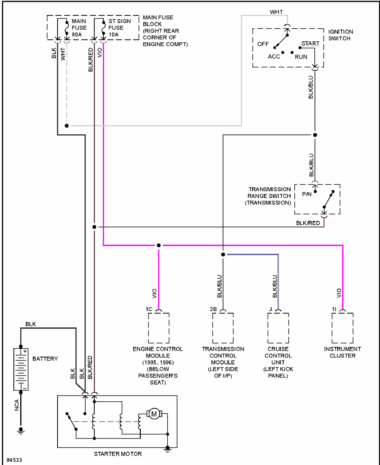
Fig. 27: Starting Circuit, A/T
