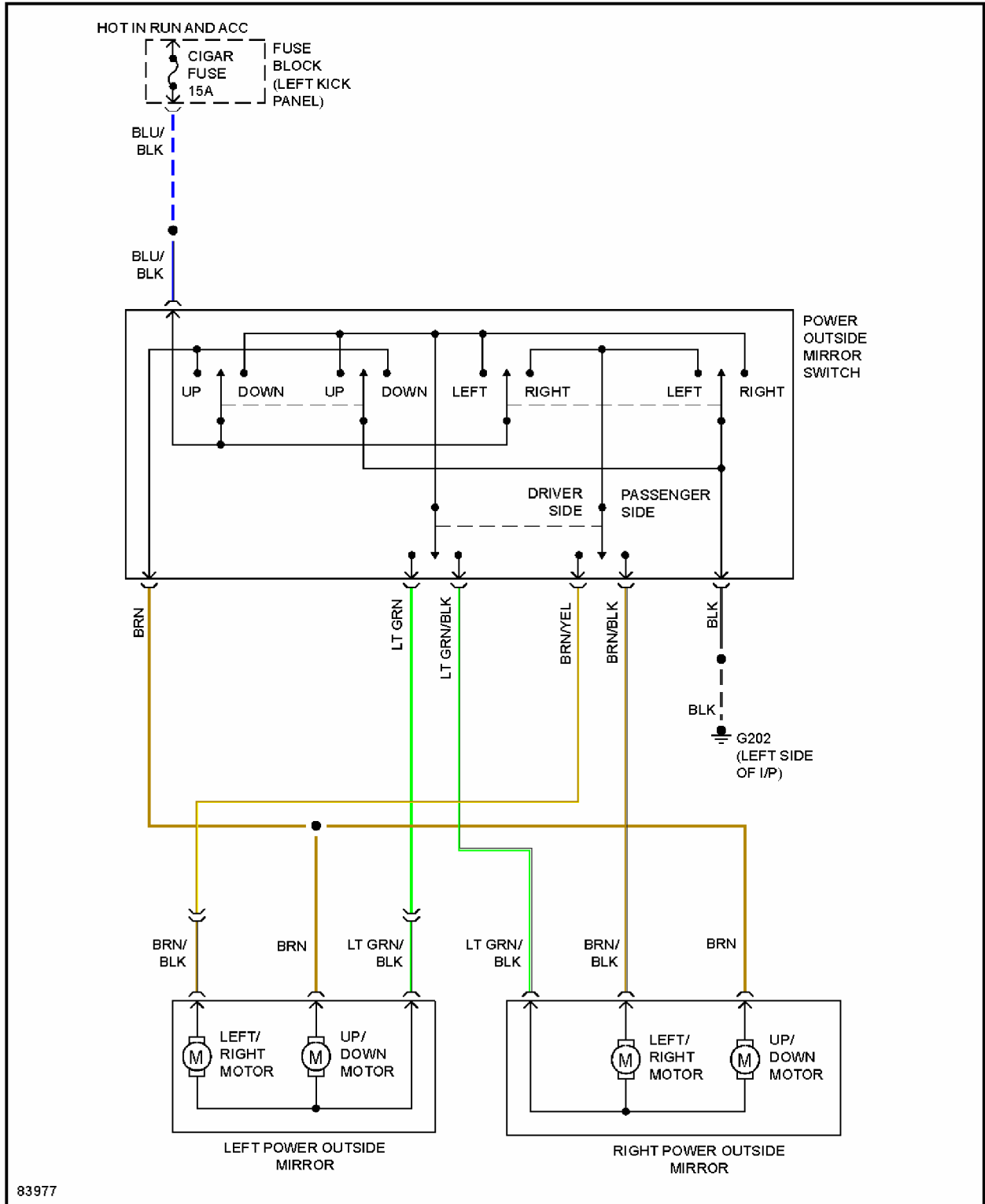
Fig. 21: Power Mirror Circuit
