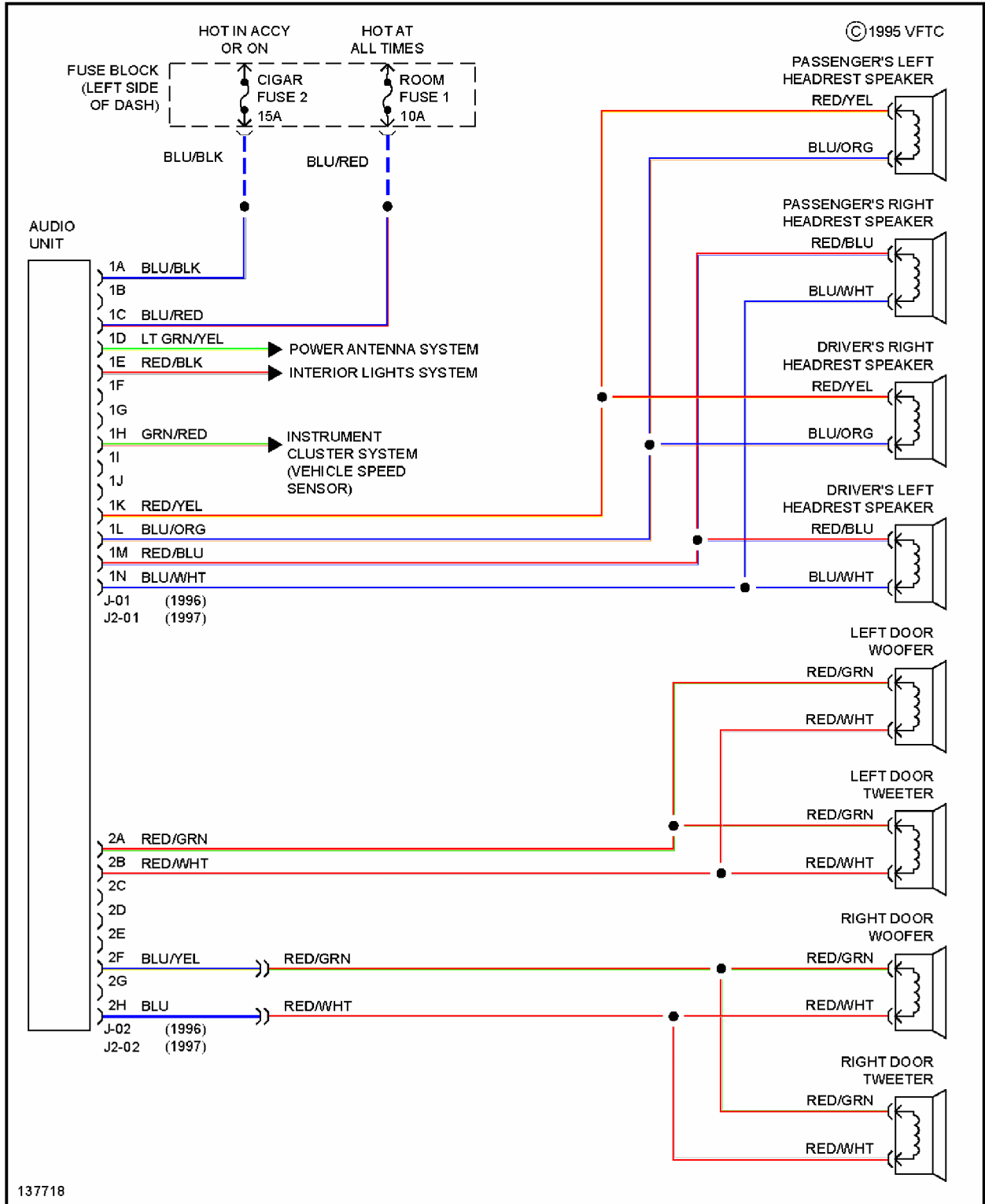
Fig. 24: Premium Sound Radio Circuit
