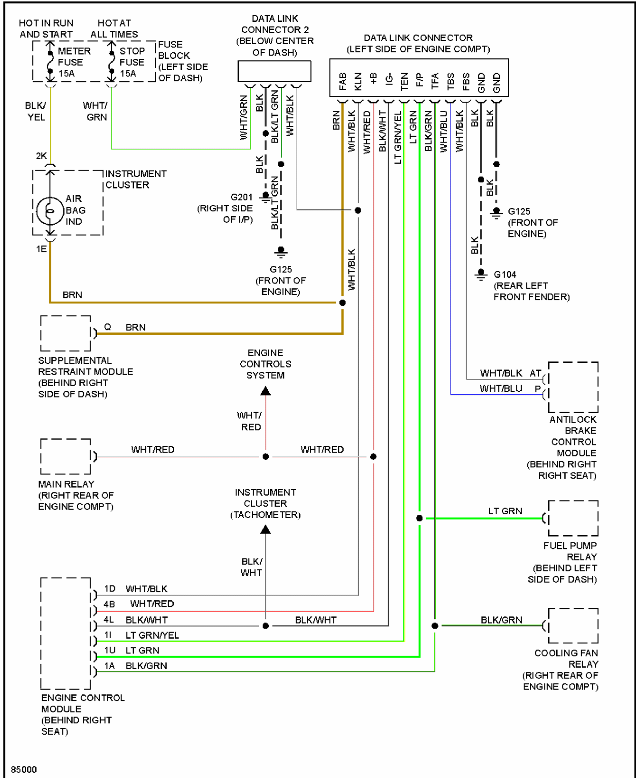
Fig. 4: Data Link Connector Circuit
