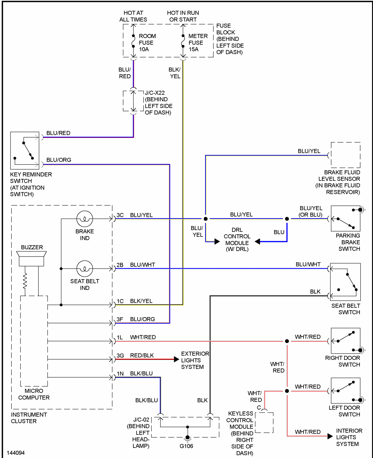
Fig. 32: Warning System Circuits
