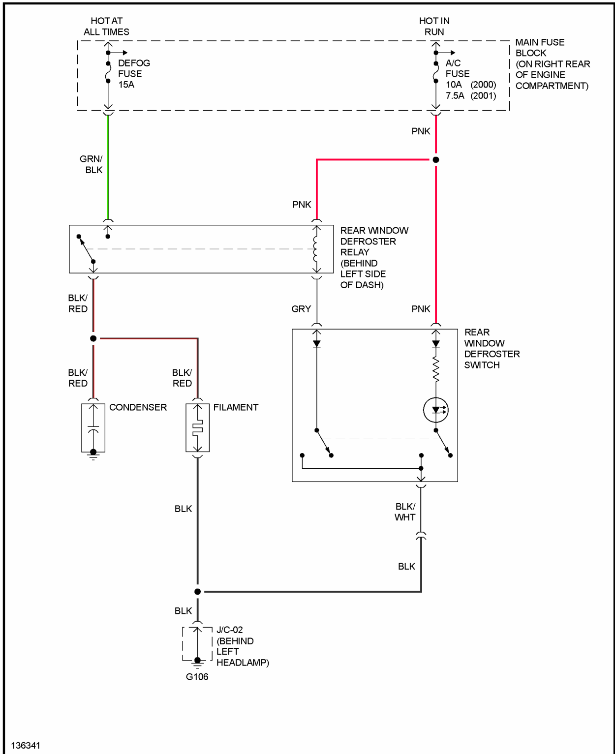
Fig. 7: Defogger Circuit
