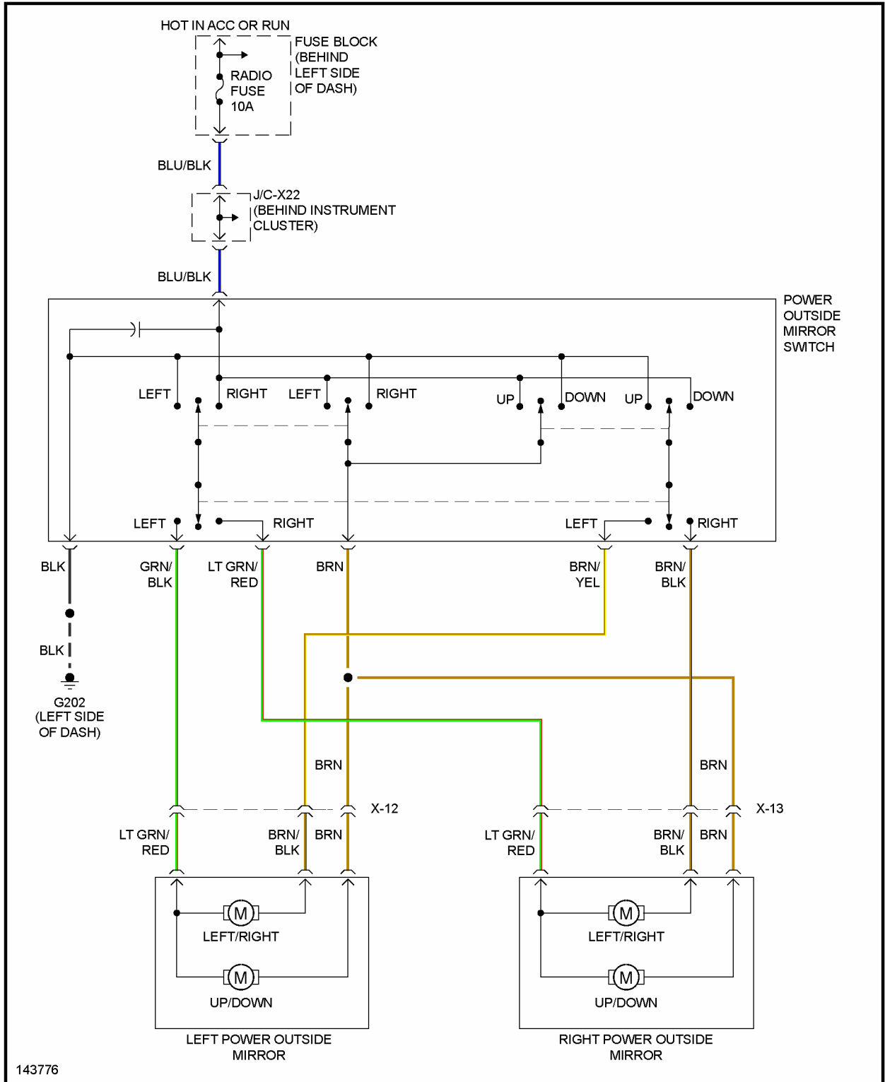
Fig. 22: Power Mirror Circuit
