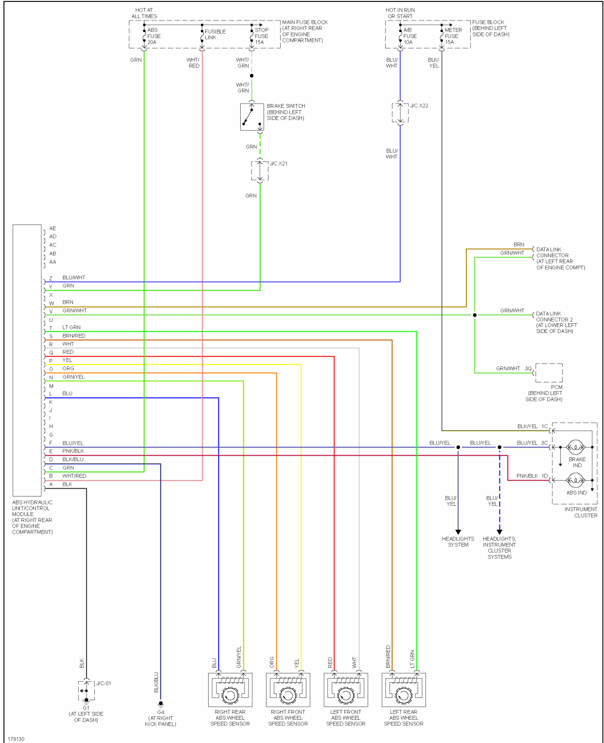
Fig. 2: Anti-lock Brakes Circuit
