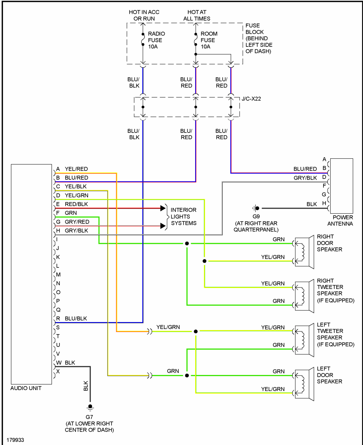
Fig. 25: Radio Circuit, Standard
