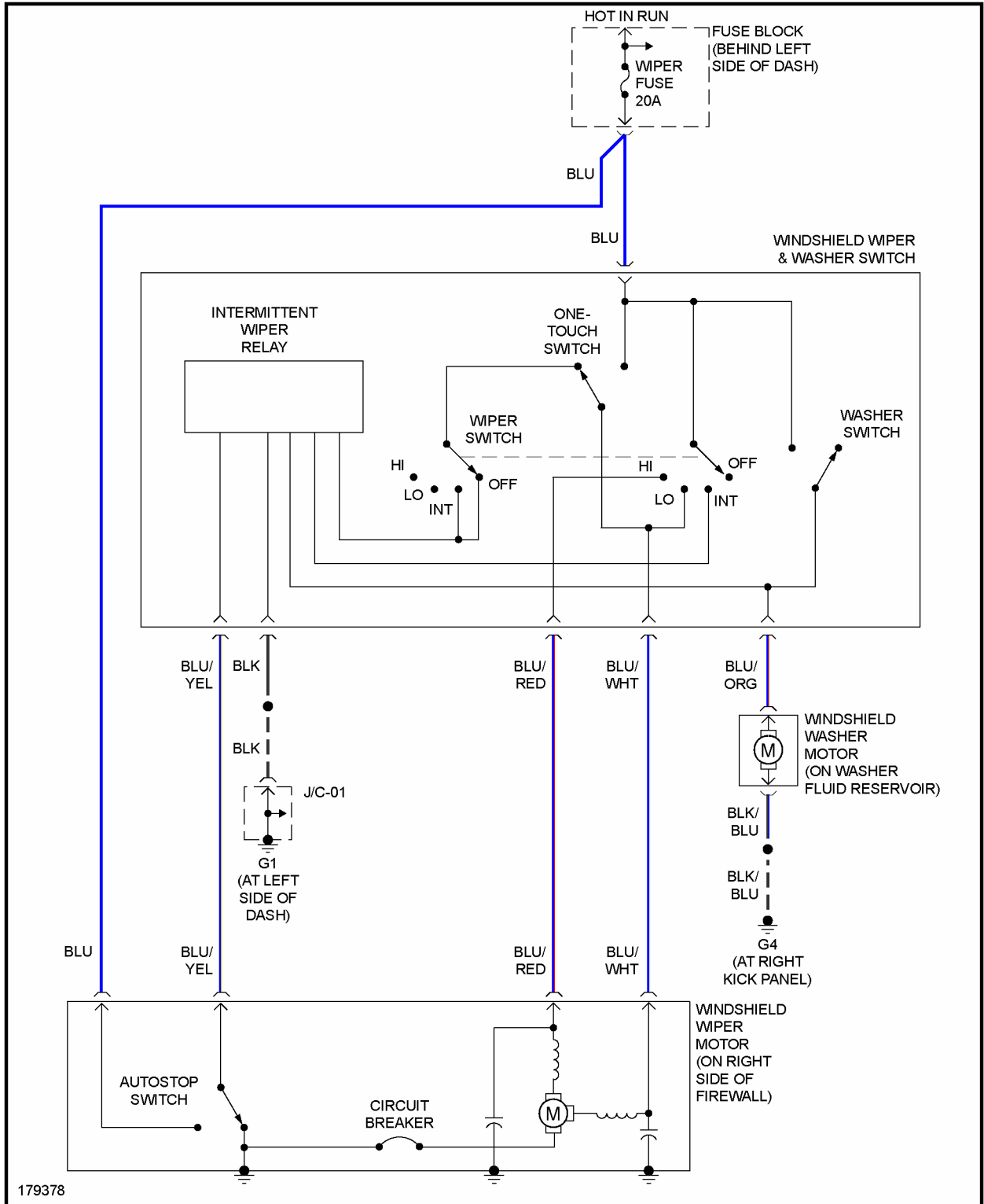
Fig. 33: Wiper/Washer Circuit
