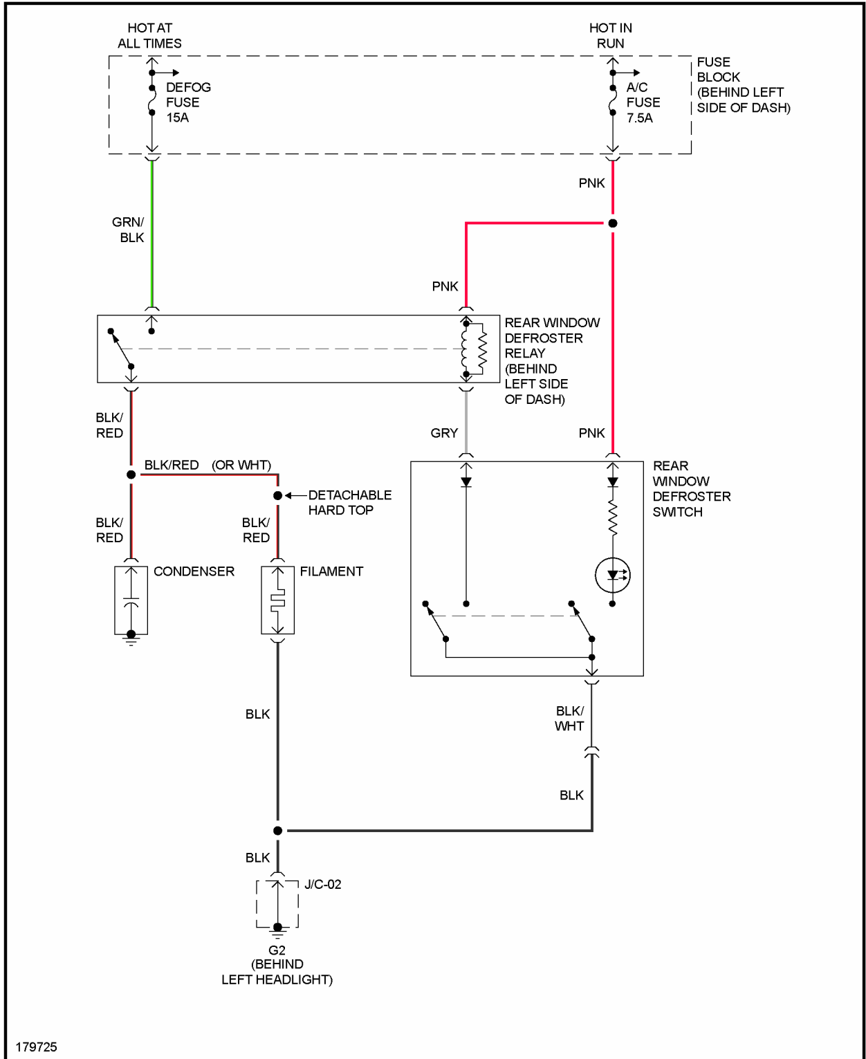
Fig. 7: Defoggers Circuit
