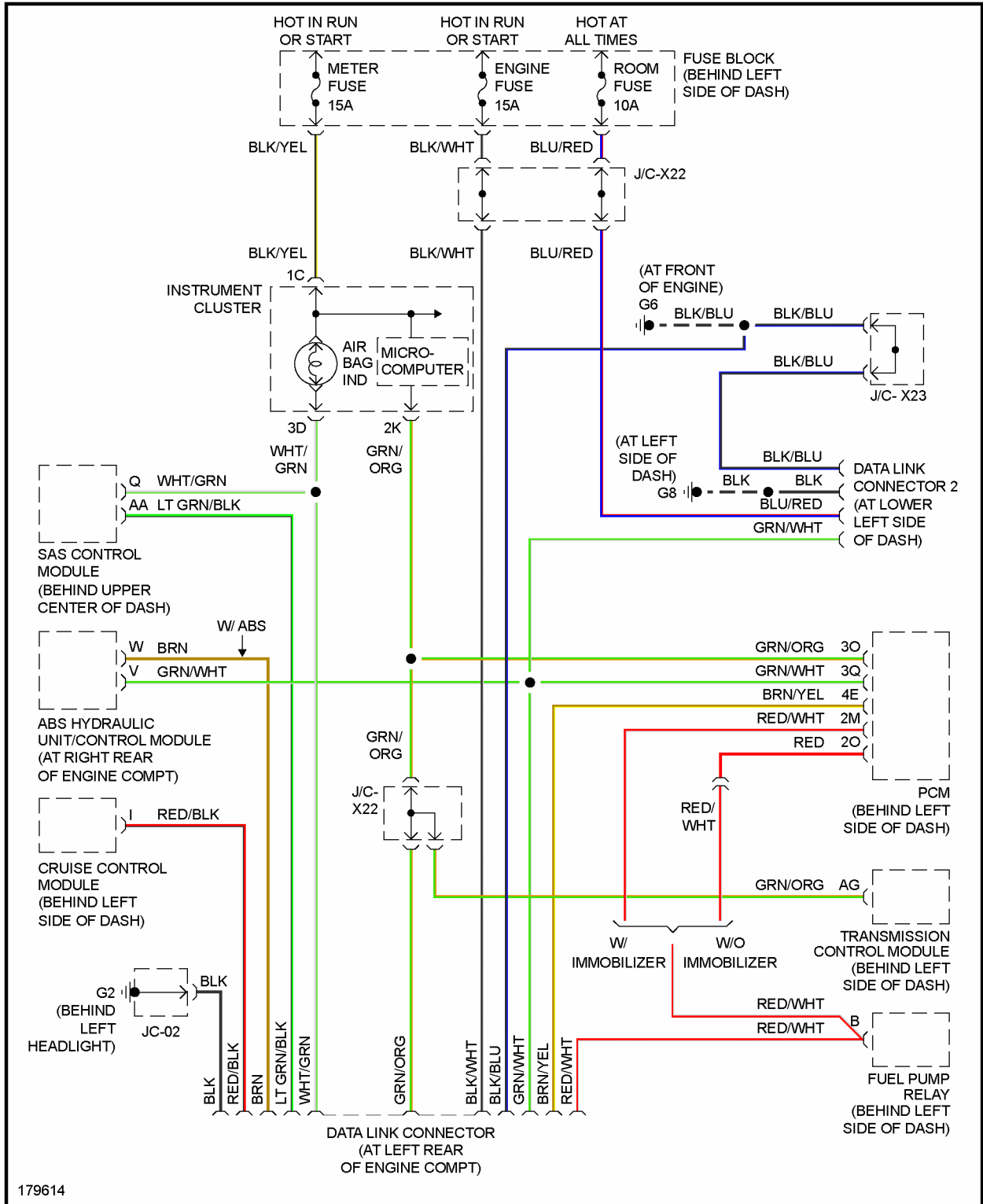
Fig. 4: Computer Data Lines Circuit
