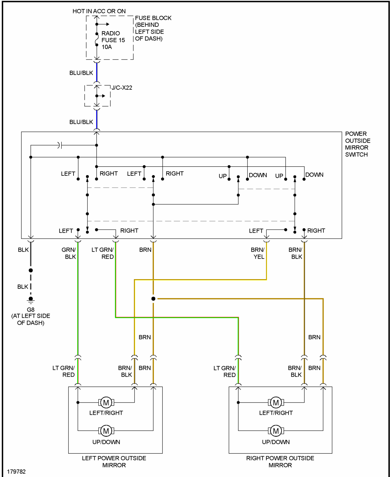
Fig. 22: Power Mirrors Circuit
