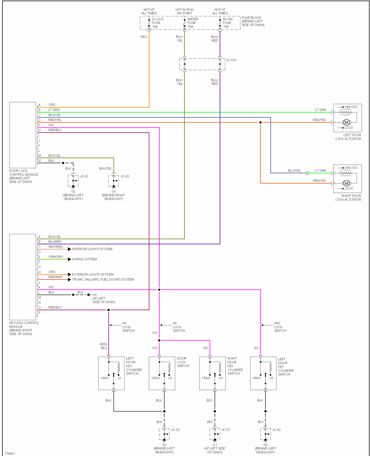
Fig. 21: Door Lock & Keyless Entry Circuit
