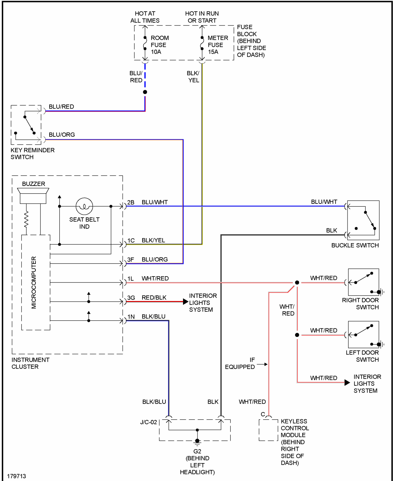
Fig. 32: Warning Systems Circuit
