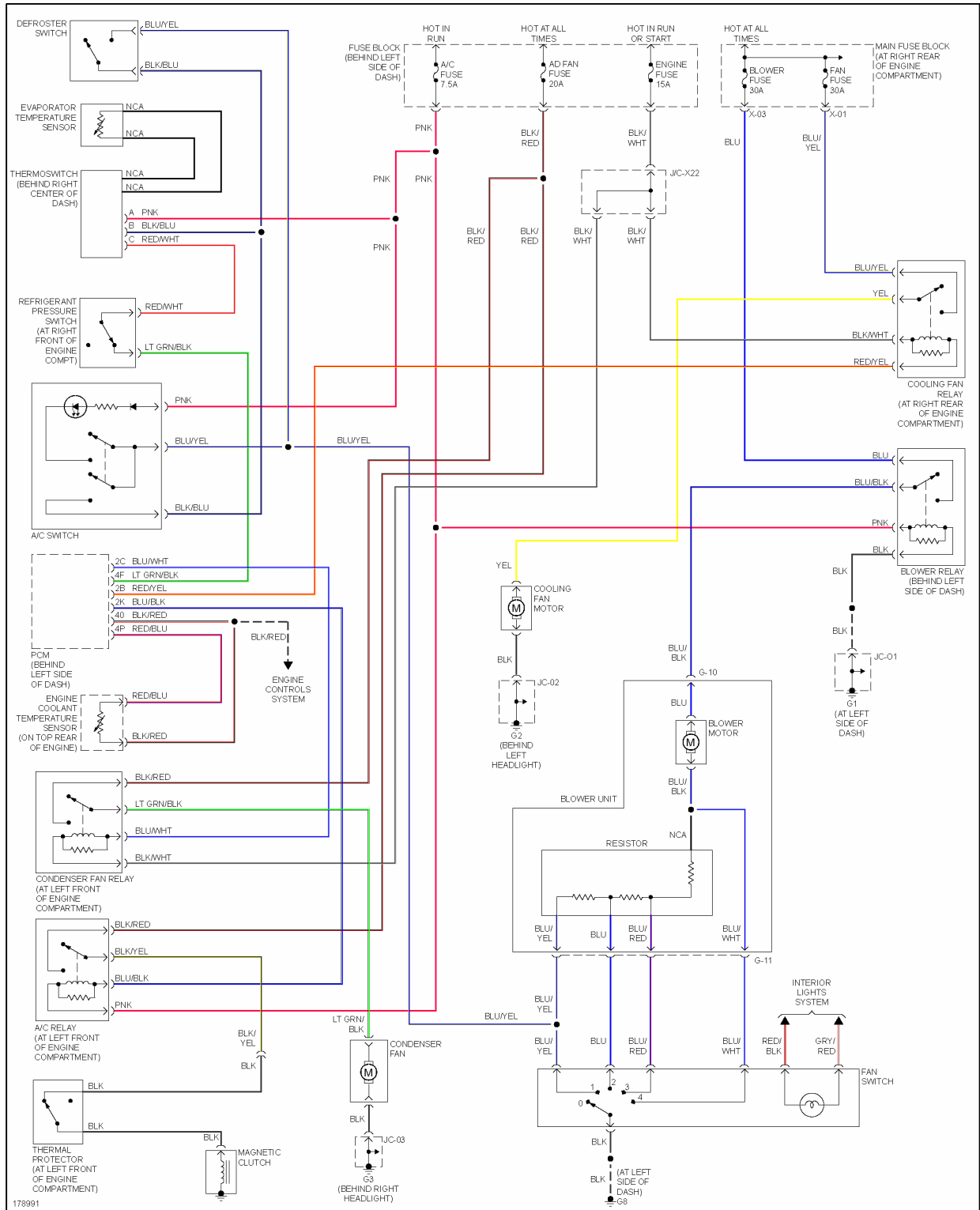
Fig. 1: Manual A/C Circuit
