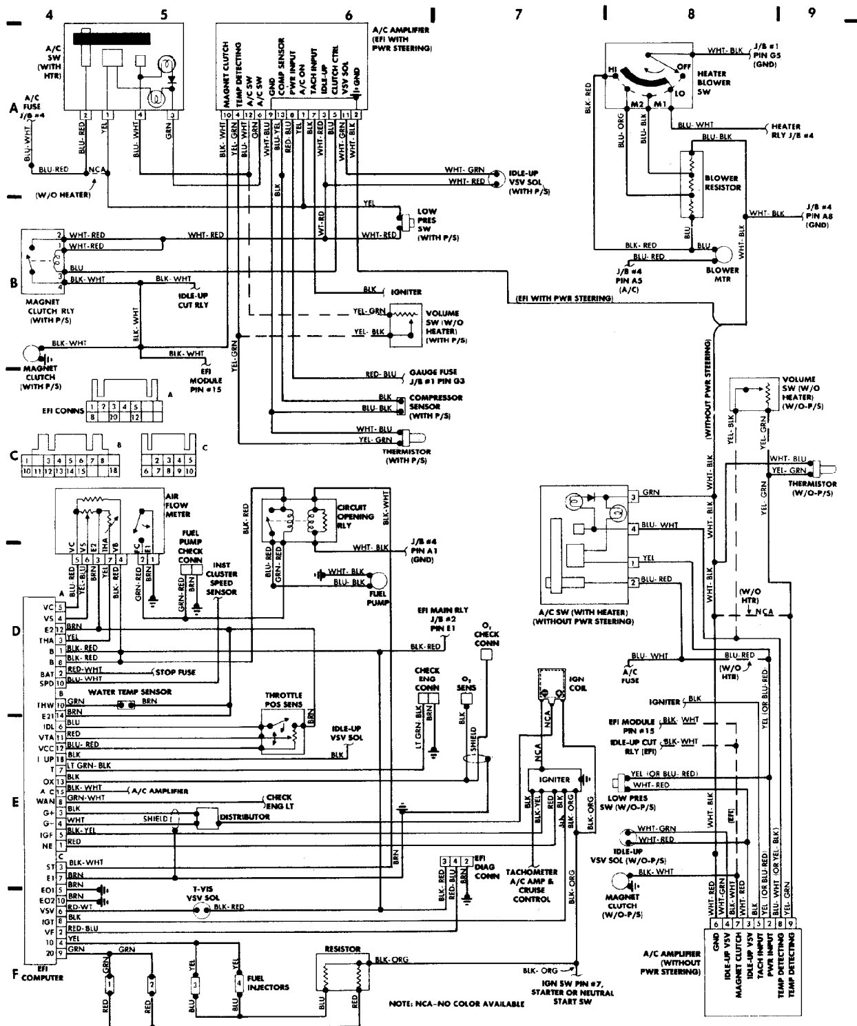
Fig. 2: Engine Compartment (Cont.) & Underdash
