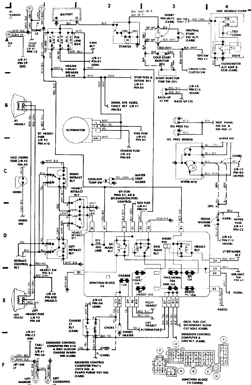
Fig. 1: Engine Compartment
