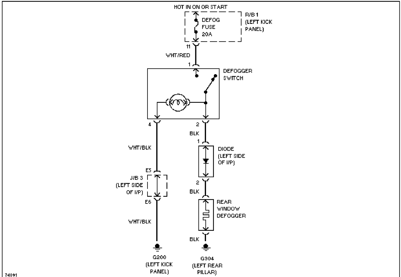
Defogger Circuit
