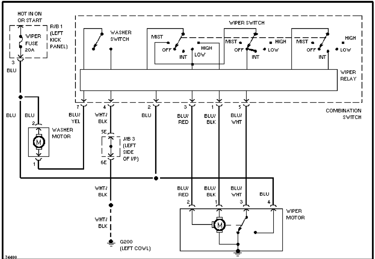
Wiper/Washer Circuit
