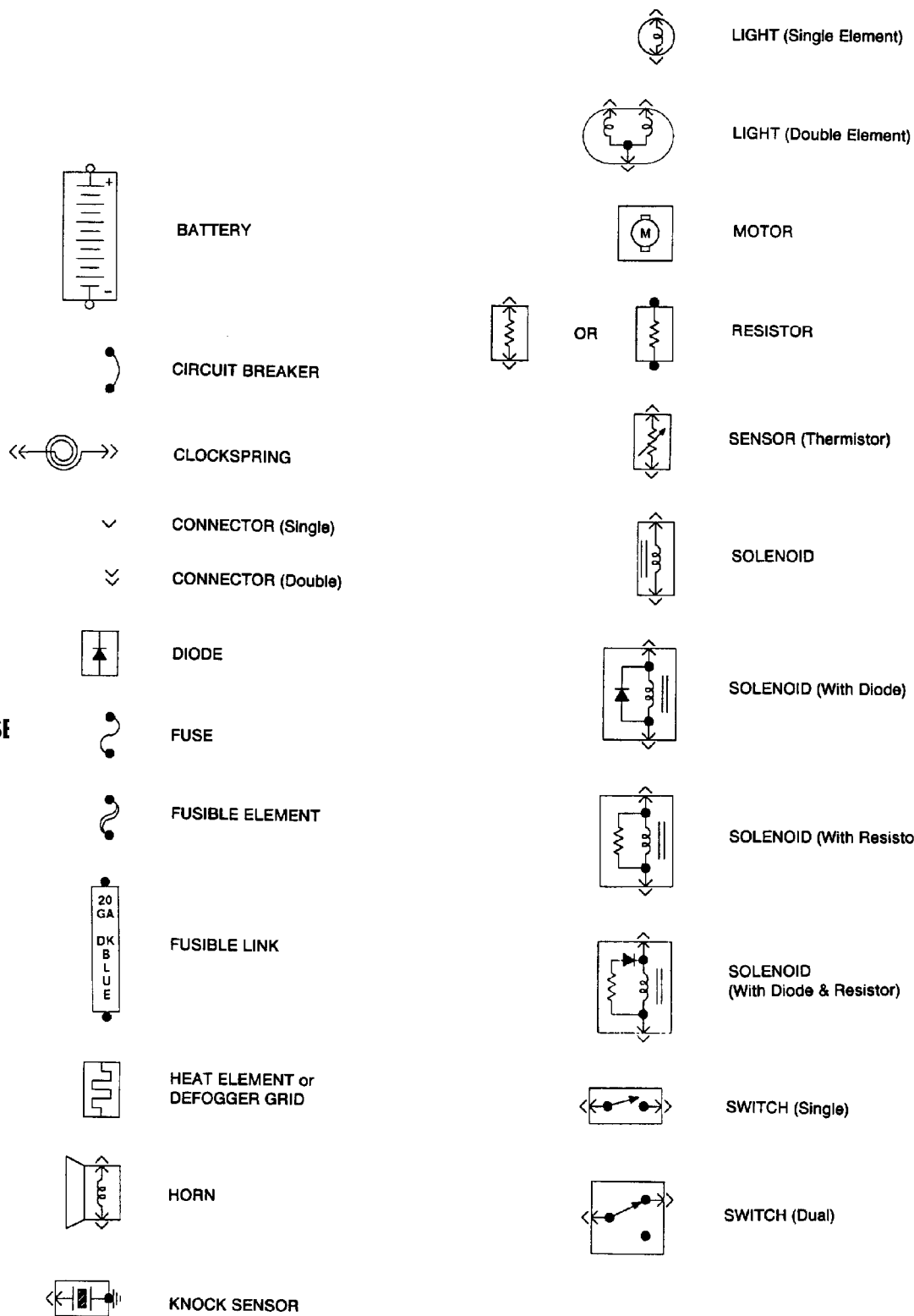
50E03637 Fig. 1: Identifying Wiring Diagram Symbols
