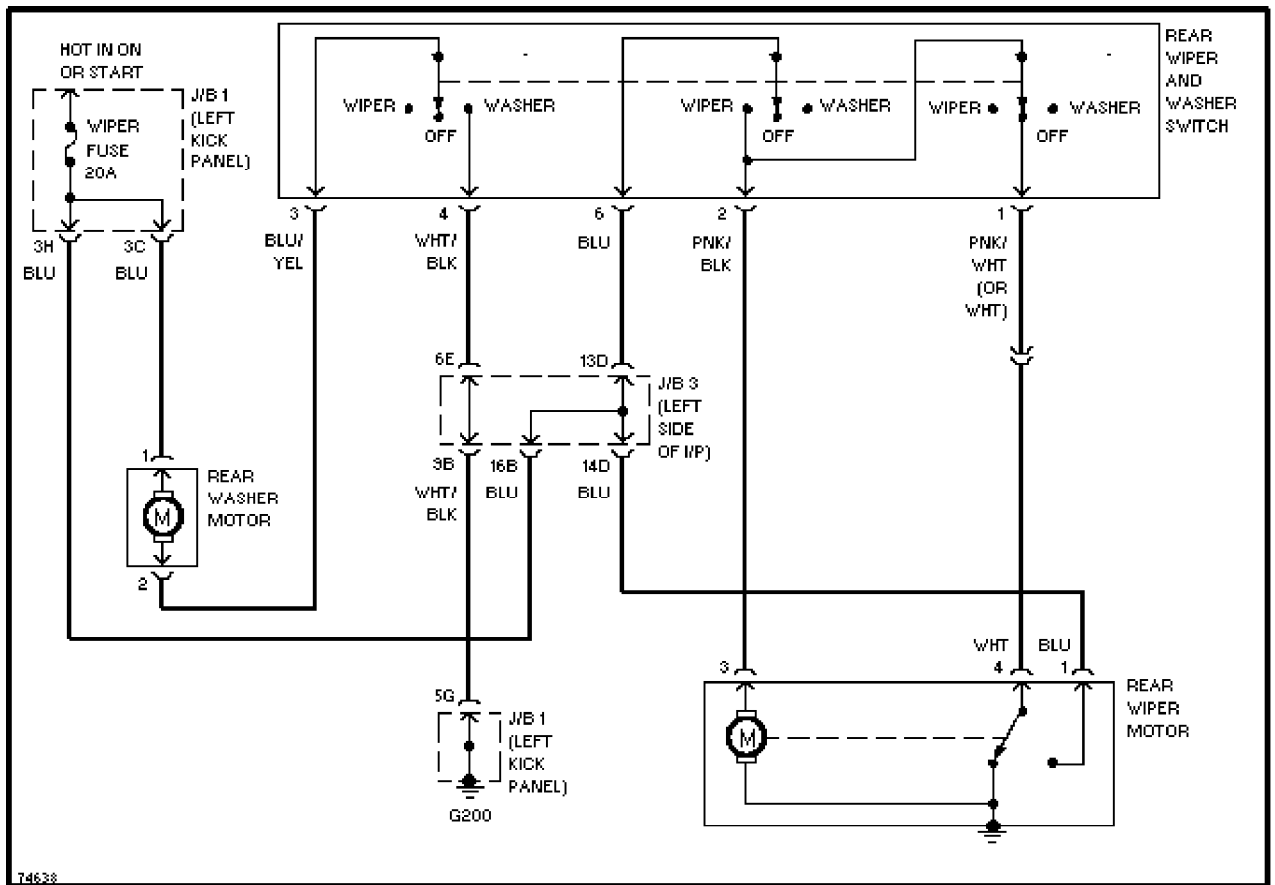
1.6L (Carb), Rear Wiper/Washer Circuit
