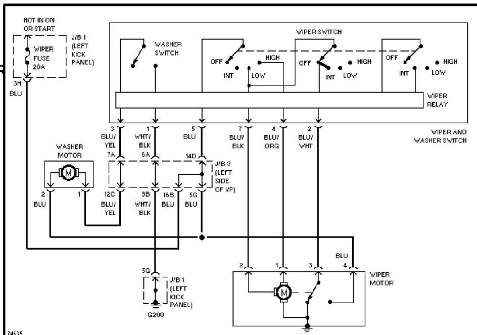
1.6L (EFI), Front Wiper/Washer Circuit
