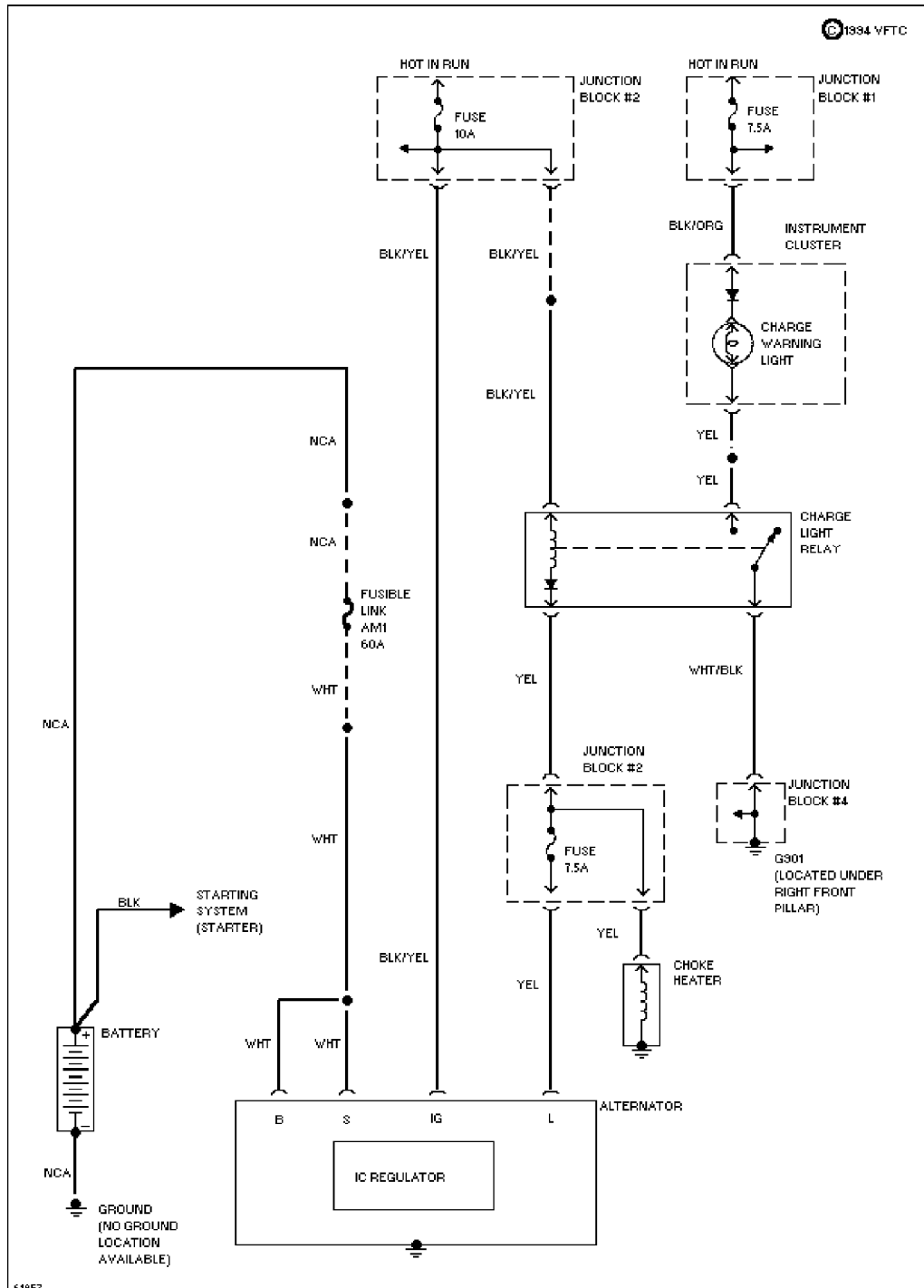
1.6L, Charging Circuit, 4A-C
