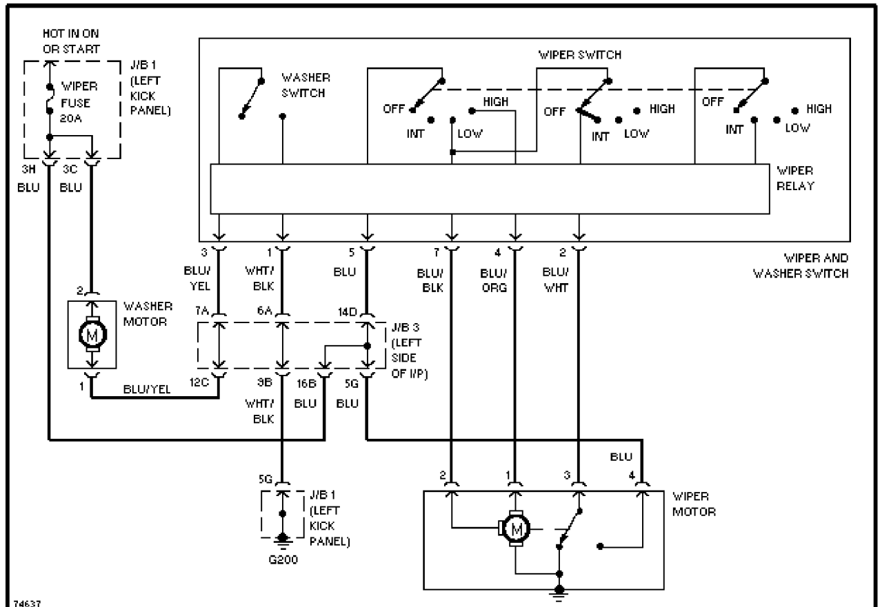
1.6L (Carb), Front Wiper/Washer Circuit
