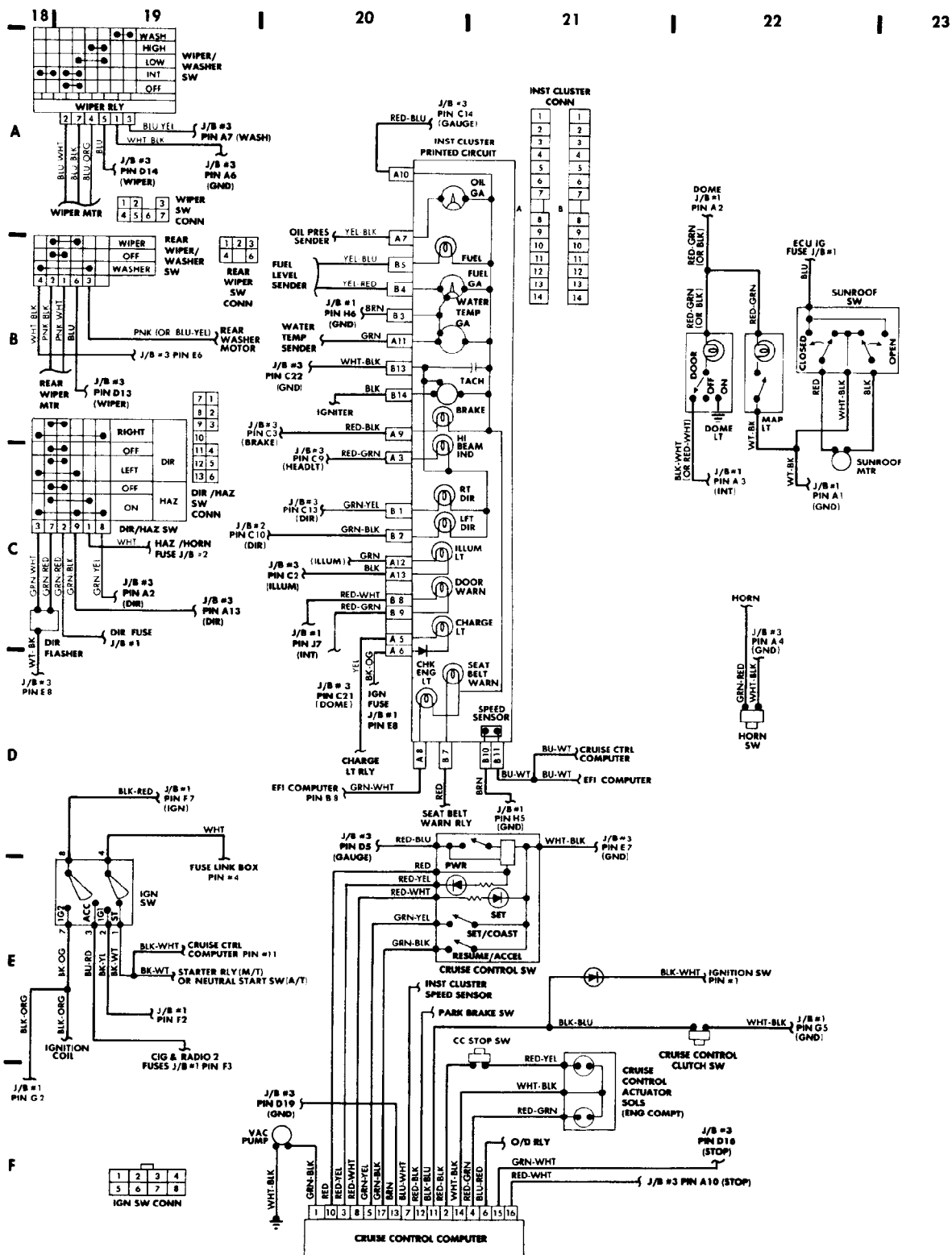
Fig. 5: Instrument Panel, Cruise Control & Passenger Compartment 1986 Toyota Corolla (RWD) For Rse 555 Main Street Clarksville Va 22901
