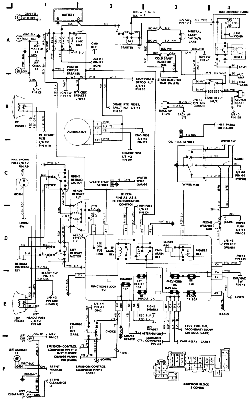
Fig. 1: Engine Compartment & Fuseblock No. 1 (Grids 1-4)
