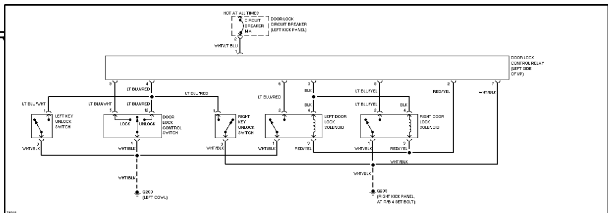
Power Door Lock Circuit
