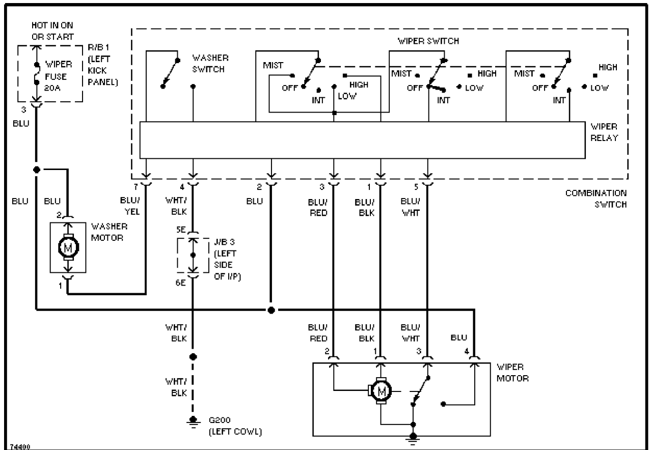
Wiper/Washer Circuit
