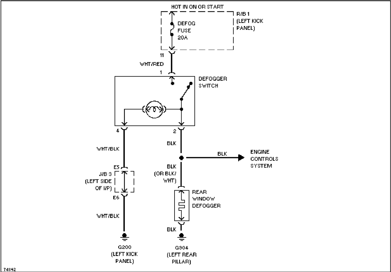
Defogger Circuit
