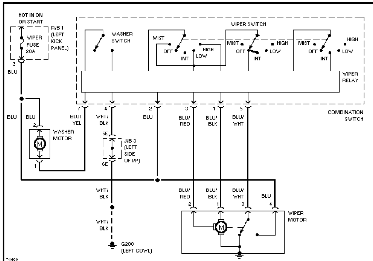
Wiper/Washer Circuit
