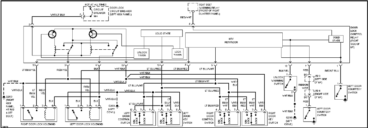
Power Door Lock Circuit
