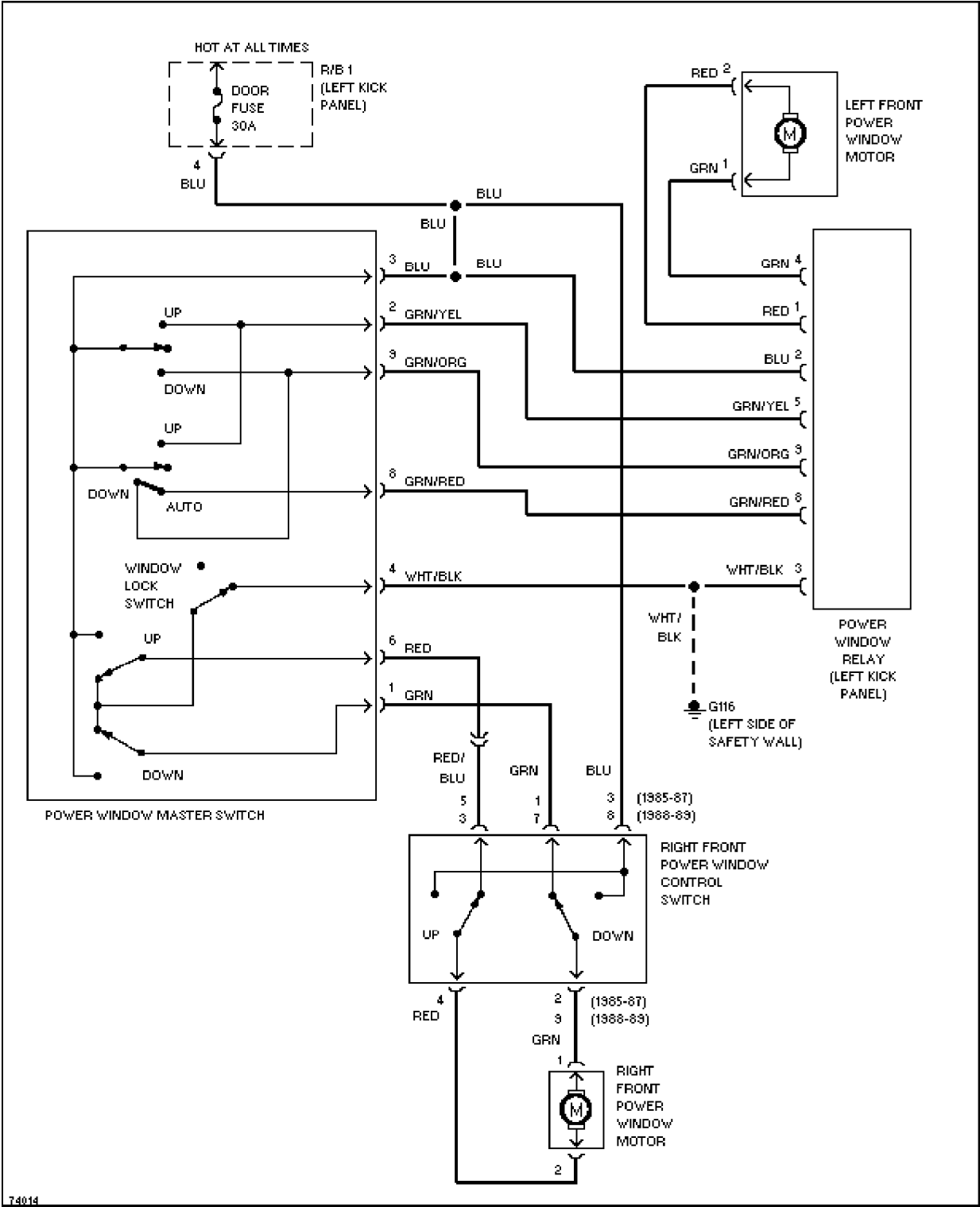
Power Window Circuit SYSTEM WIRING DIAGRAMS Article Text (p. 8) 1989 Toyota MR2 For Ace Mechanics 123 Main Street San Diego Ca 9
