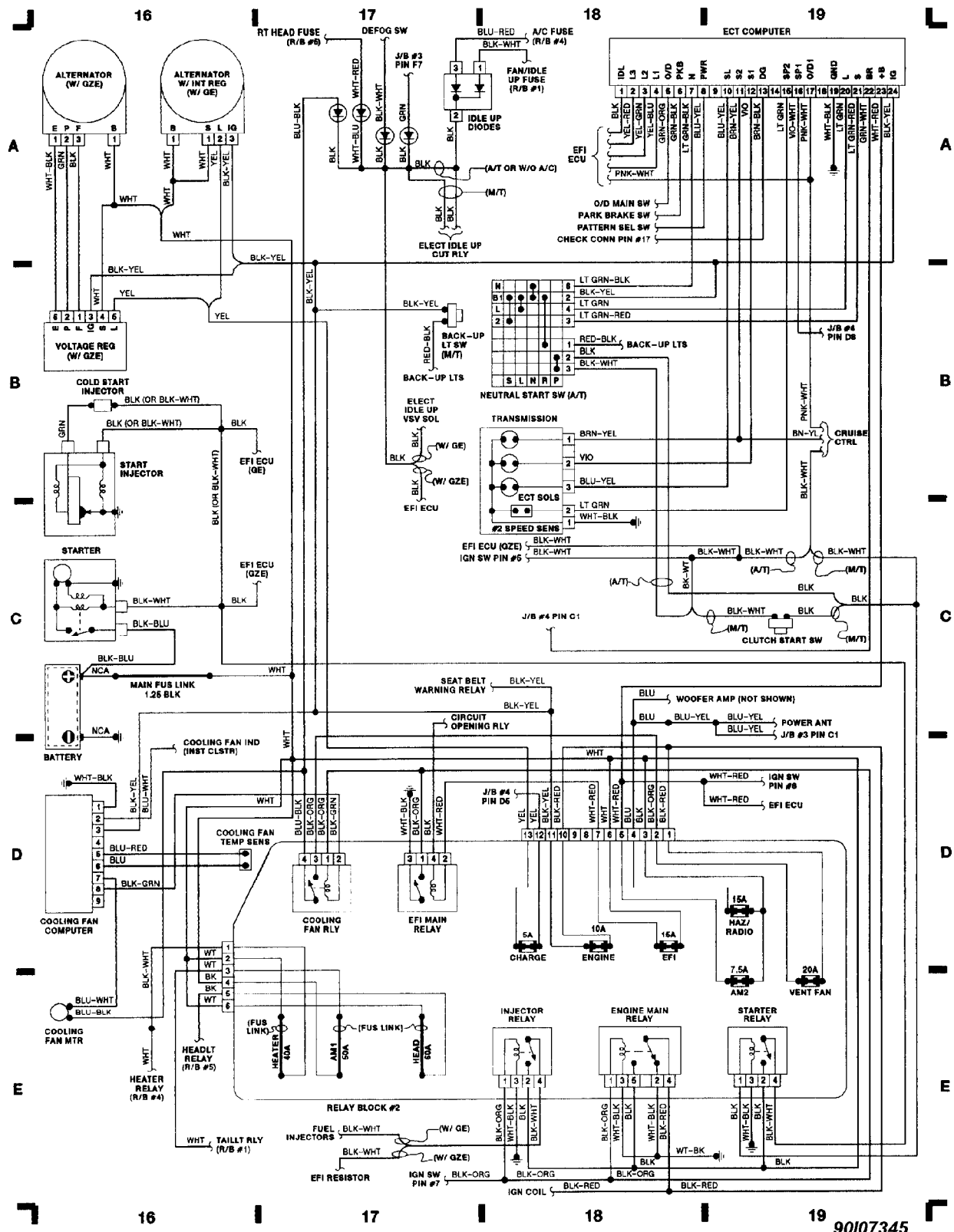
Fig. 5: Automatic Transmission Control and Fuse Block No. 2 WIRING DIAGRAMS Article Text (p. 7) 1989 Toyota MR2 For Ace Mechanics 123 Main Street San Diego Ca 92126 Copyright
