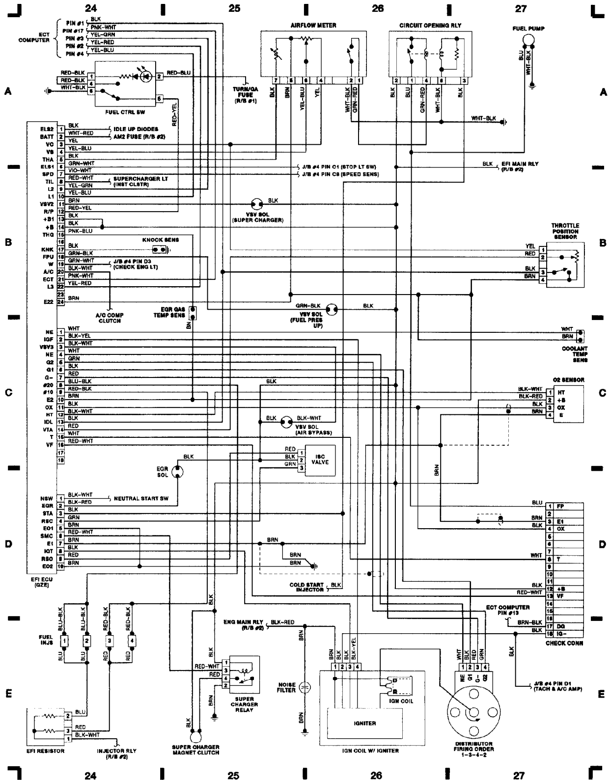
Fig. 7: Computer Engine Control (Supercharged)
