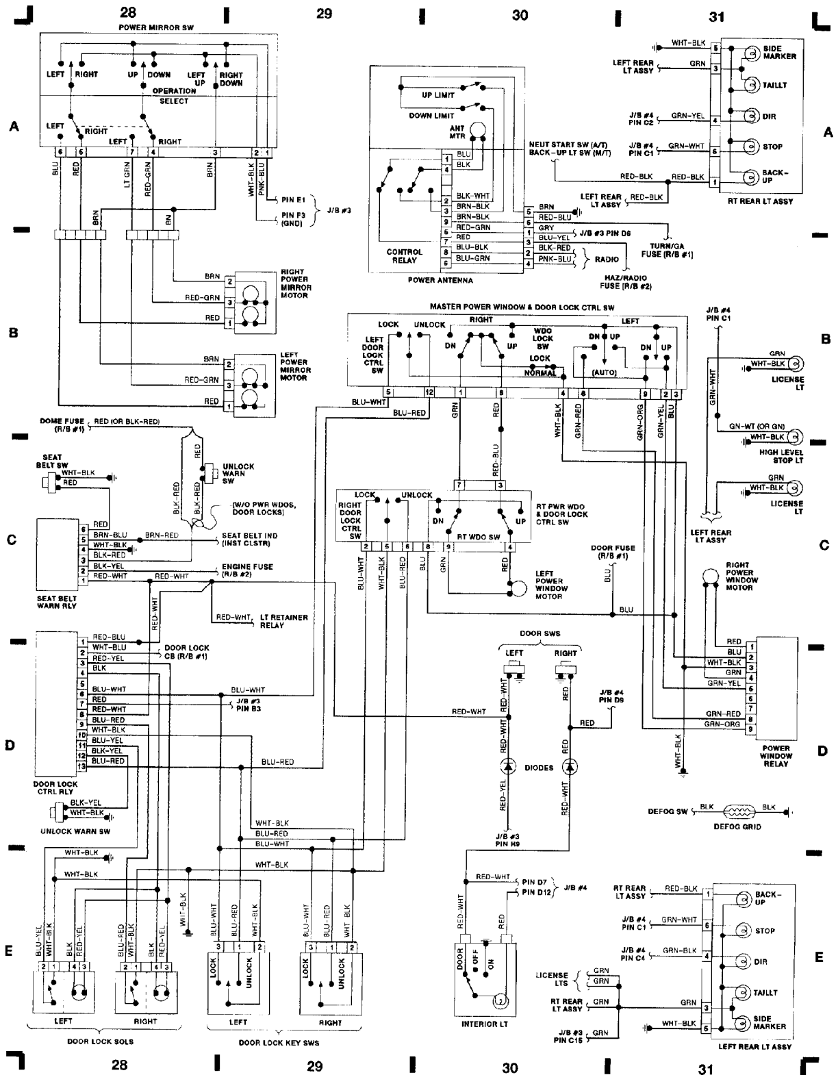
Fig. 8: Engine Compartment and Taillights
