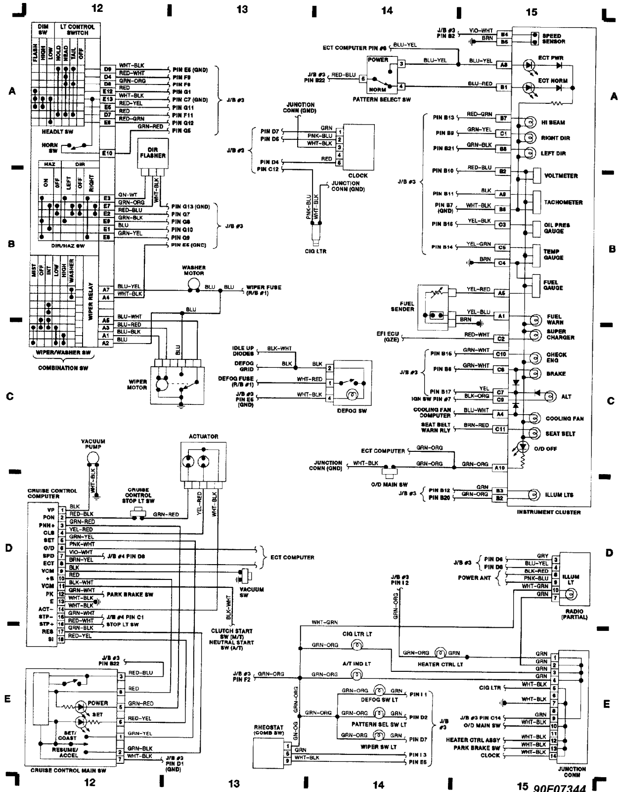
Fig. 4: Steering Column, Cruise Control and Instrument Panel WIRING DIAGRAMS Article Text (p. 6) 1989 Toyota MR2 For Ace Mechanics 123 Main Street San Diego Ca 92126 Copyright
