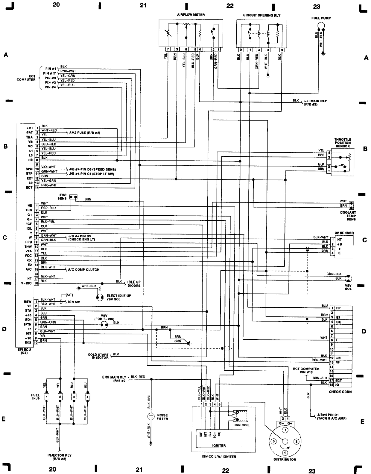
Fig. 6: Computer Engine Control (Non-Supercharged)
