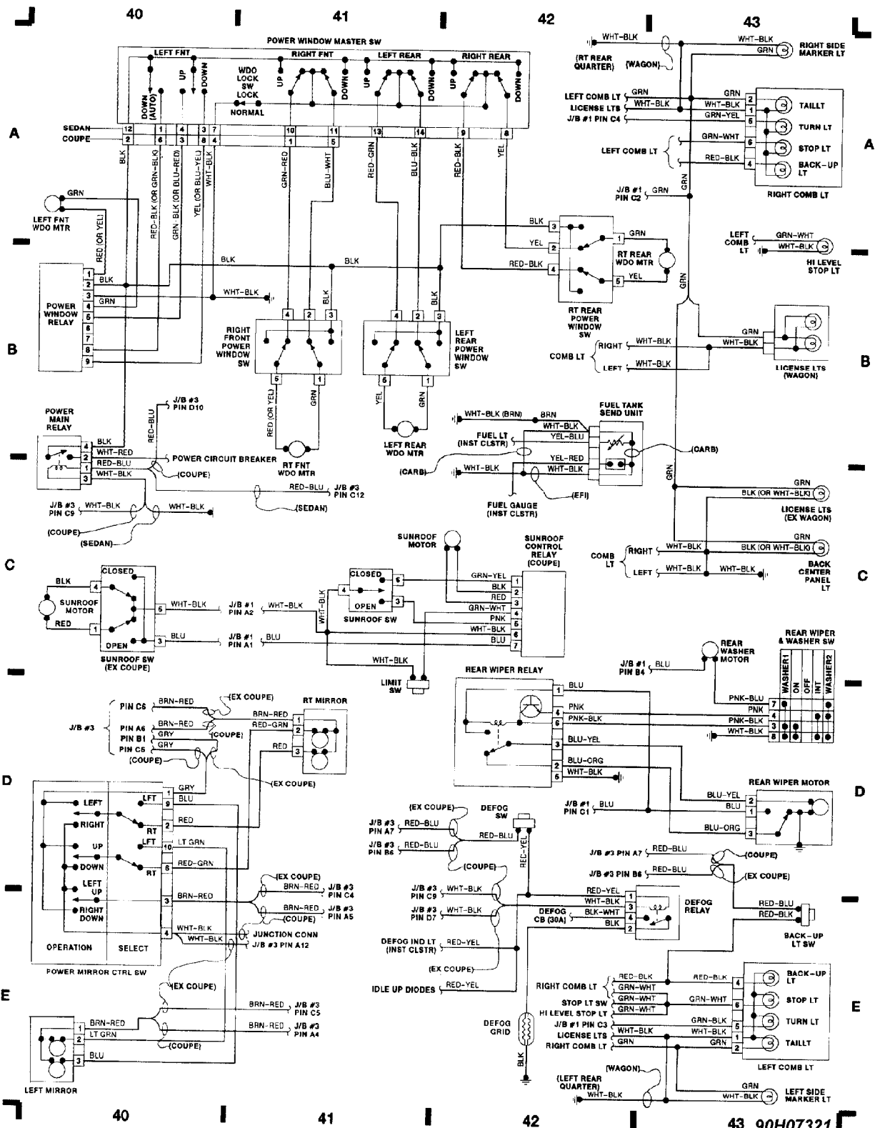
Fig. 11: Passenger Compartment & Taillights
