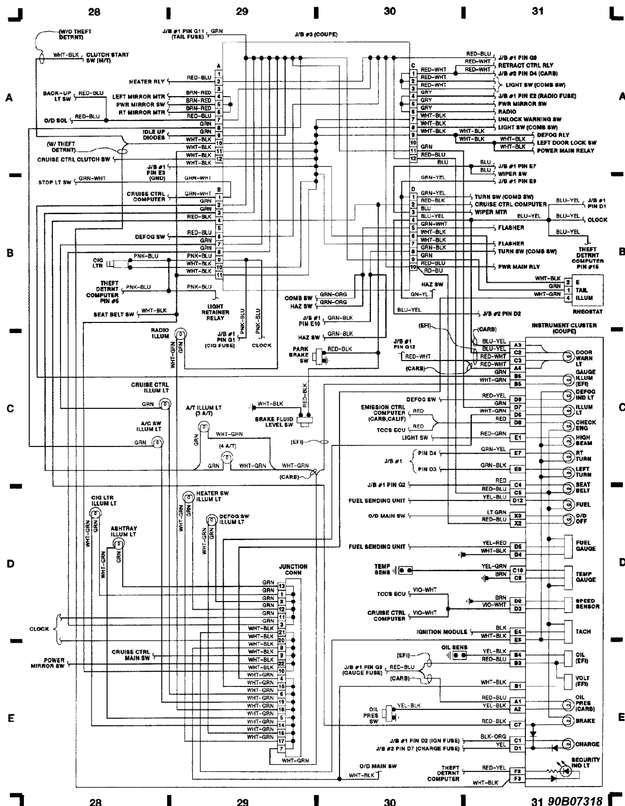
Fig. 8: Instrument Panel and Fuse Block No. 3 (Coupe)
