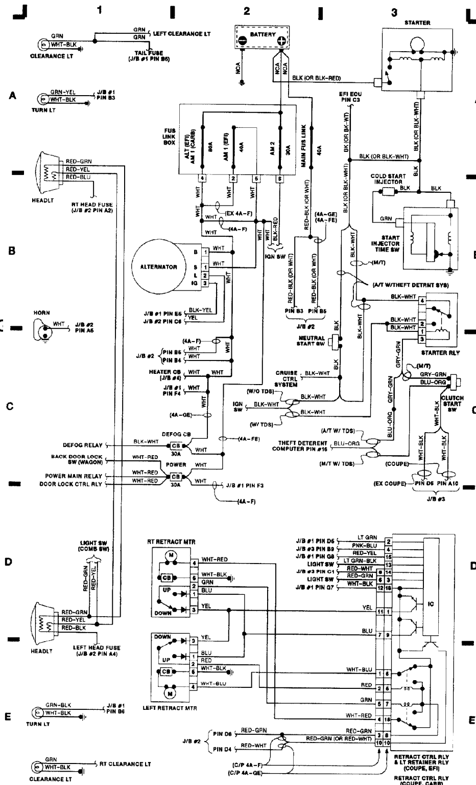
Fig. 1: Engine Compartment & Headlights
