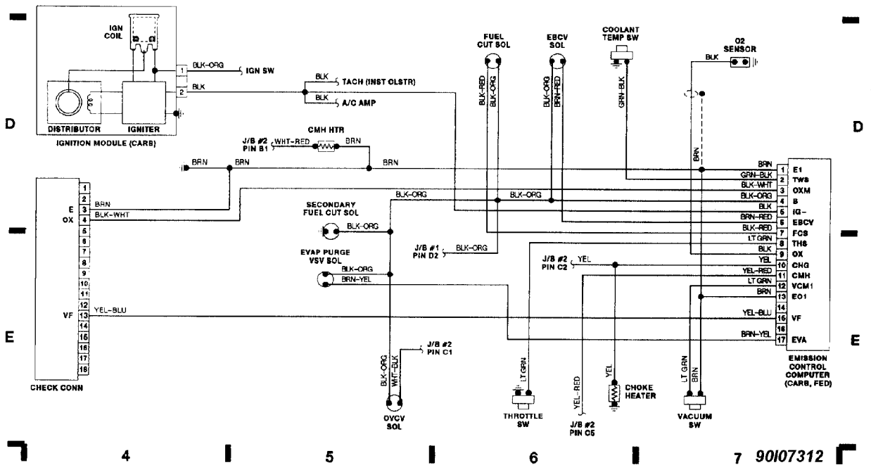
Fig. 2: Computer Engine Control (Carbureted)
