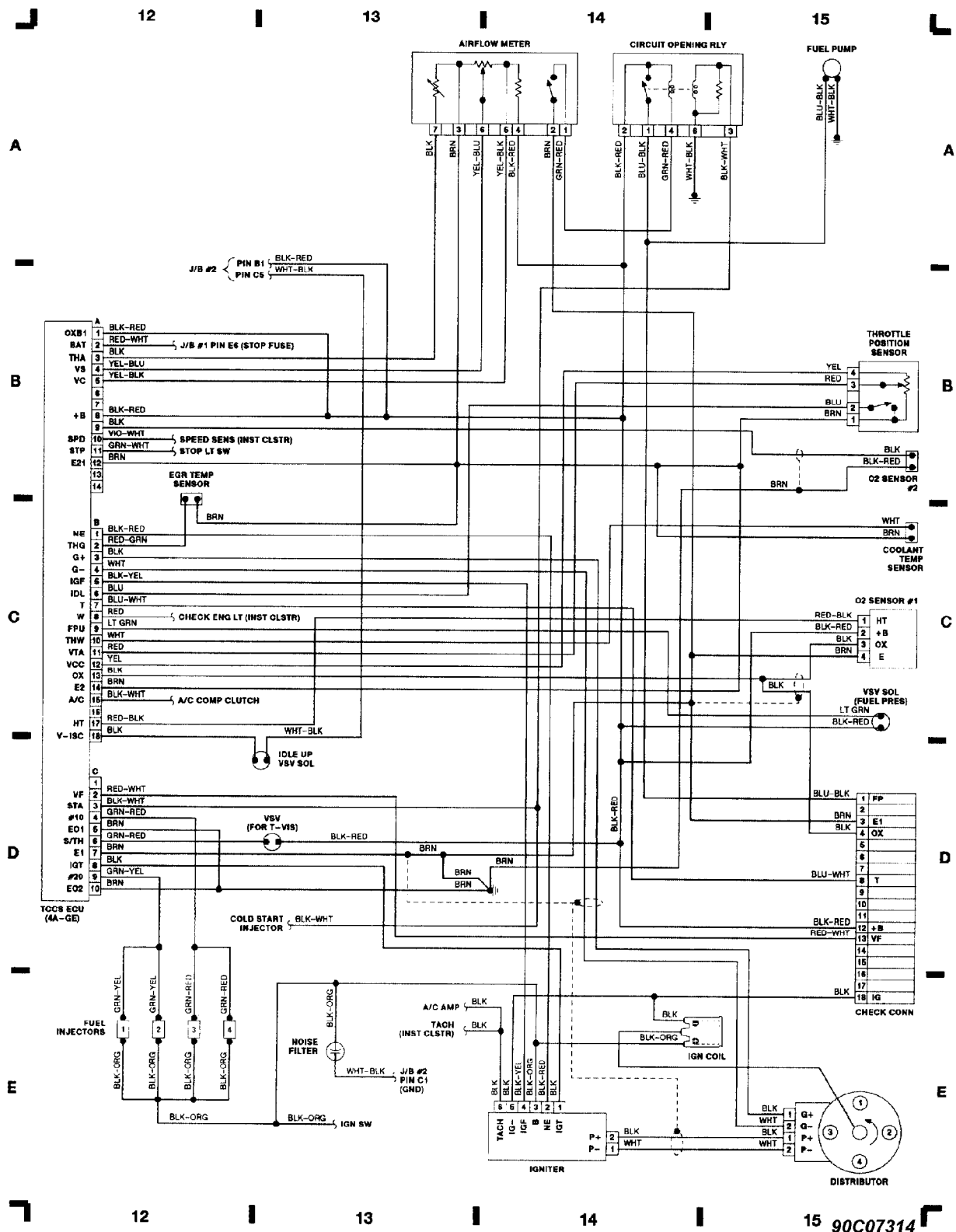
Fig. 4: Computer Engine Control (Fuel Injected GE)
