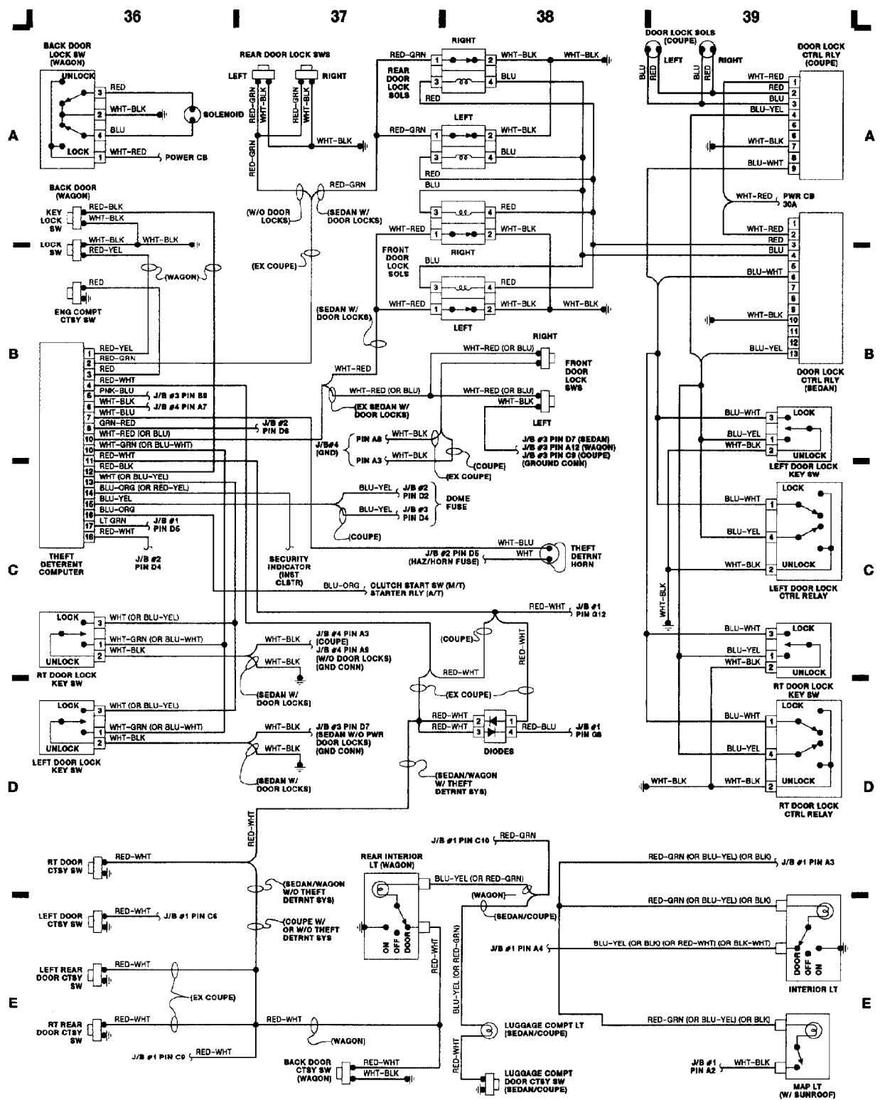
Fig. 10: Anti-Theft System and Power Door Locks WIRING DIAGRAMS Article Text (p. 13) 1989 Toyota Corolla For Rse 555 Main Street Clarksville Va 22901 Copyright
