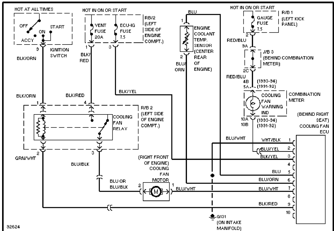
Engine Compartment Cooling Fan Circuit
