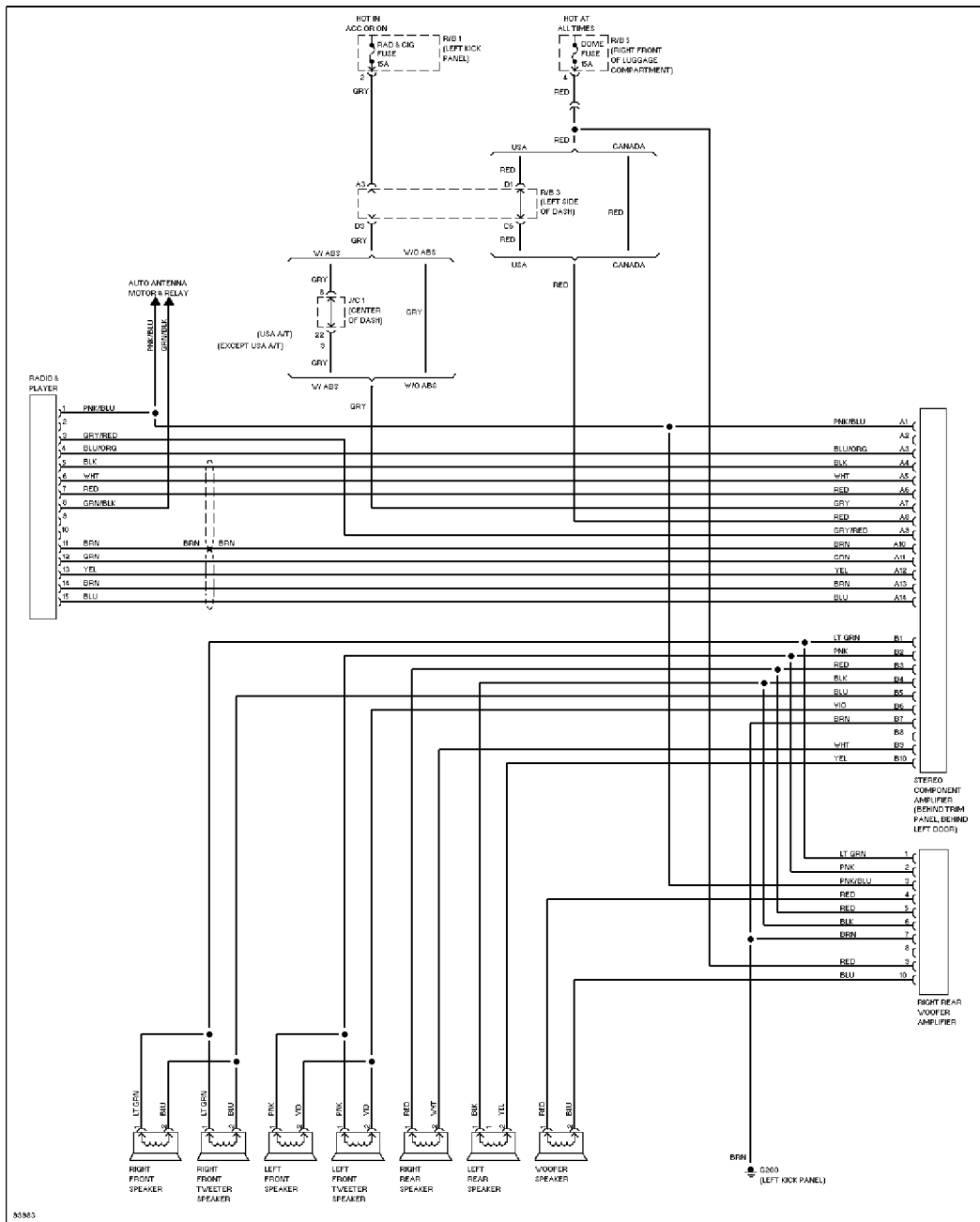
Radio Circuits, W/ CD Player
