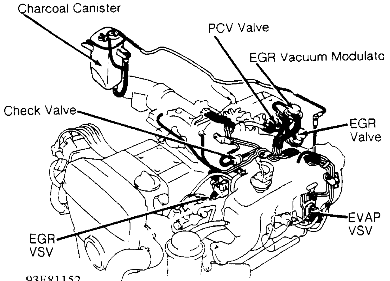
Fig. 22: Vacuum Diagram (Supra Non-Turbo - Routing) Courtesy of Toyota Motor Sales, U.S.A., Inc.
