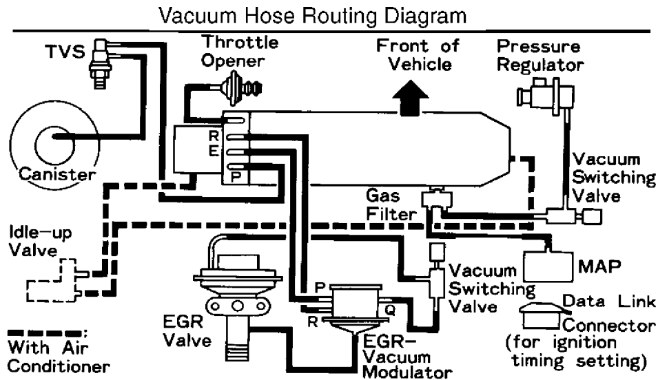
Fig. 11: Vacuum Diagram (MR2 Non-Turbo) Courtesy of Toyota Motor Sales, U.S.A., Inc.
