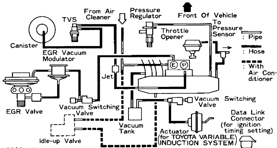
Fig. 12: Vacuum Diagram (MR2 Turbo) Courtesy of Toyota Motor Sales, U.S.A., Inc.
