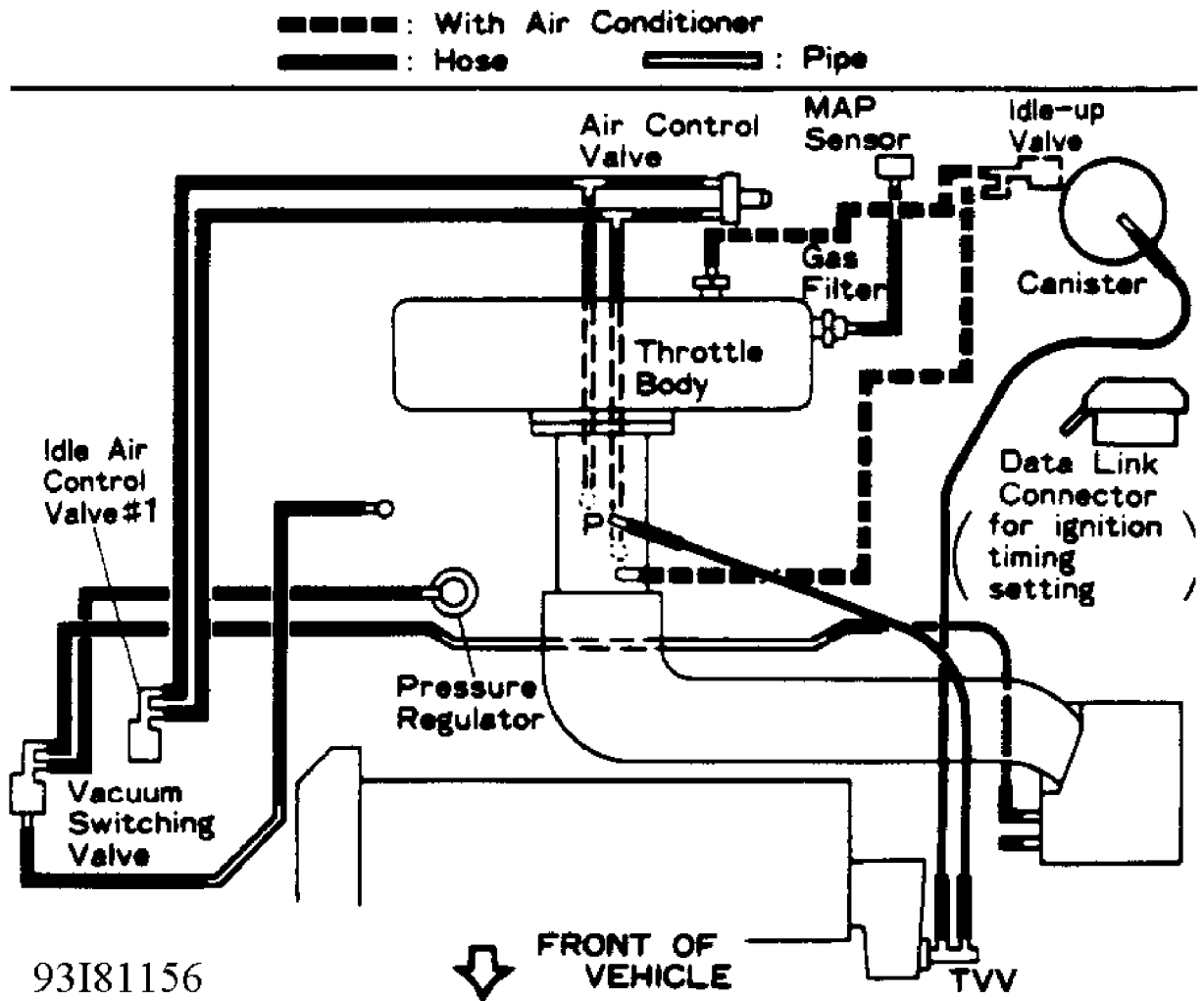
Fig. 26: Vacuum Diagram (Tercel - Federal Models W/ Power Steering)
