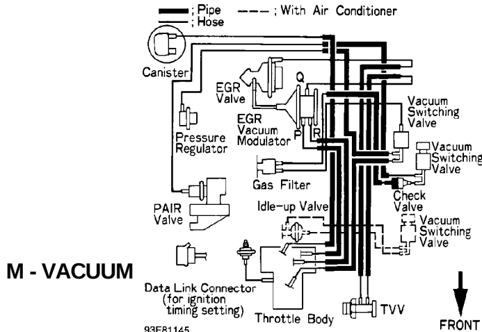
93E81145 Fig. 16: Vacuum Diagram (Pickup 2.4L & 4Runner 2.4L - Federal A/T) Courtesy of Toyota Motor Sales, U.S.A., Inc.
