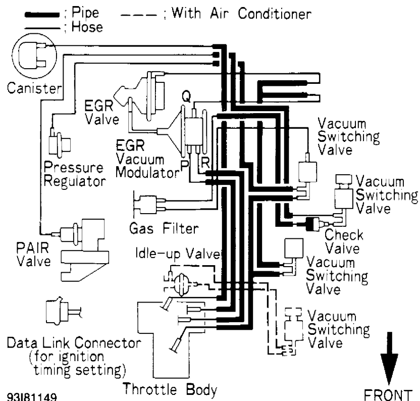
93181149 Fig. 19: Vacuum Diagram (Pickup 2.4L & 4Runner 2.4L - California M/T)
