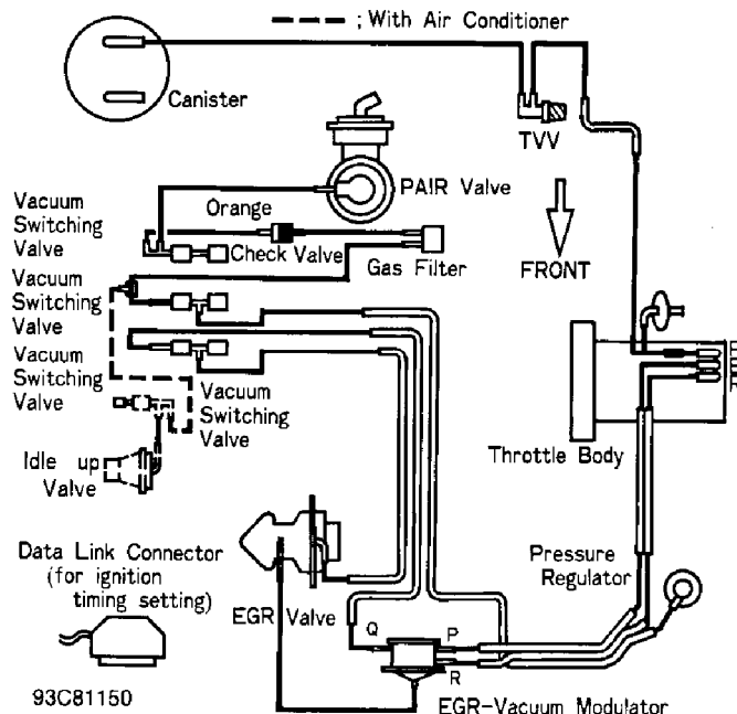
93C81150 Fig. 20: Vacuum Diagram (Pickup 3.0L & 4Runner 3.0L)
