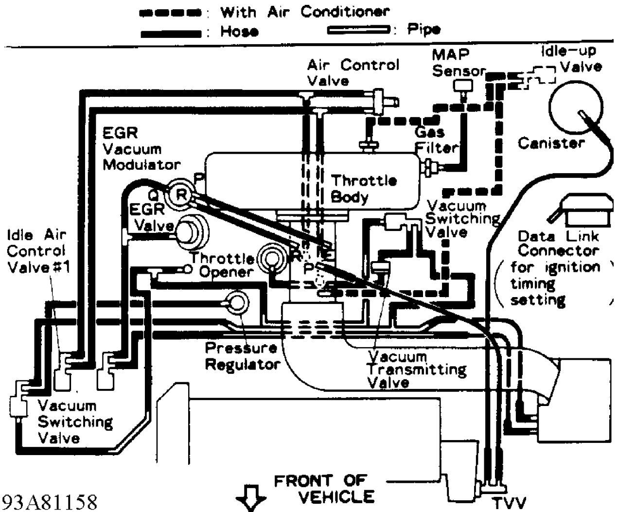
Fig. 28: Vacuum Diagram (Tercel - Calif. Models w/ Power Steering) M. VACUUM DIAGRAMS Article Text (p. 20) 1993 Toyota MR2 For Ace Mechanics 123 Main Street San Diego Ca 9212 Courtesy of Toyota Motor Sales, U.S.A., Inc.
