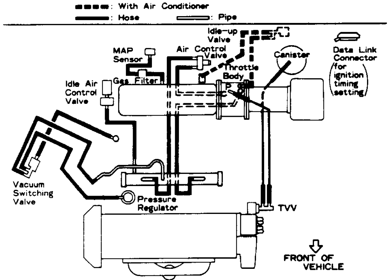
93D81144 Fig. 15: Vacuum Diagram (Paseo - California Models) Courtesy of Toyota Motor Sales, U.S.A., Inc.
