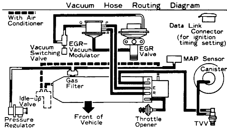
93C81135 Fig. 6: Vacuum Diagram (Celica 2.2L 5S-FE) Courtesy of Toyota Motor Sales, U.S.A., Inc.
