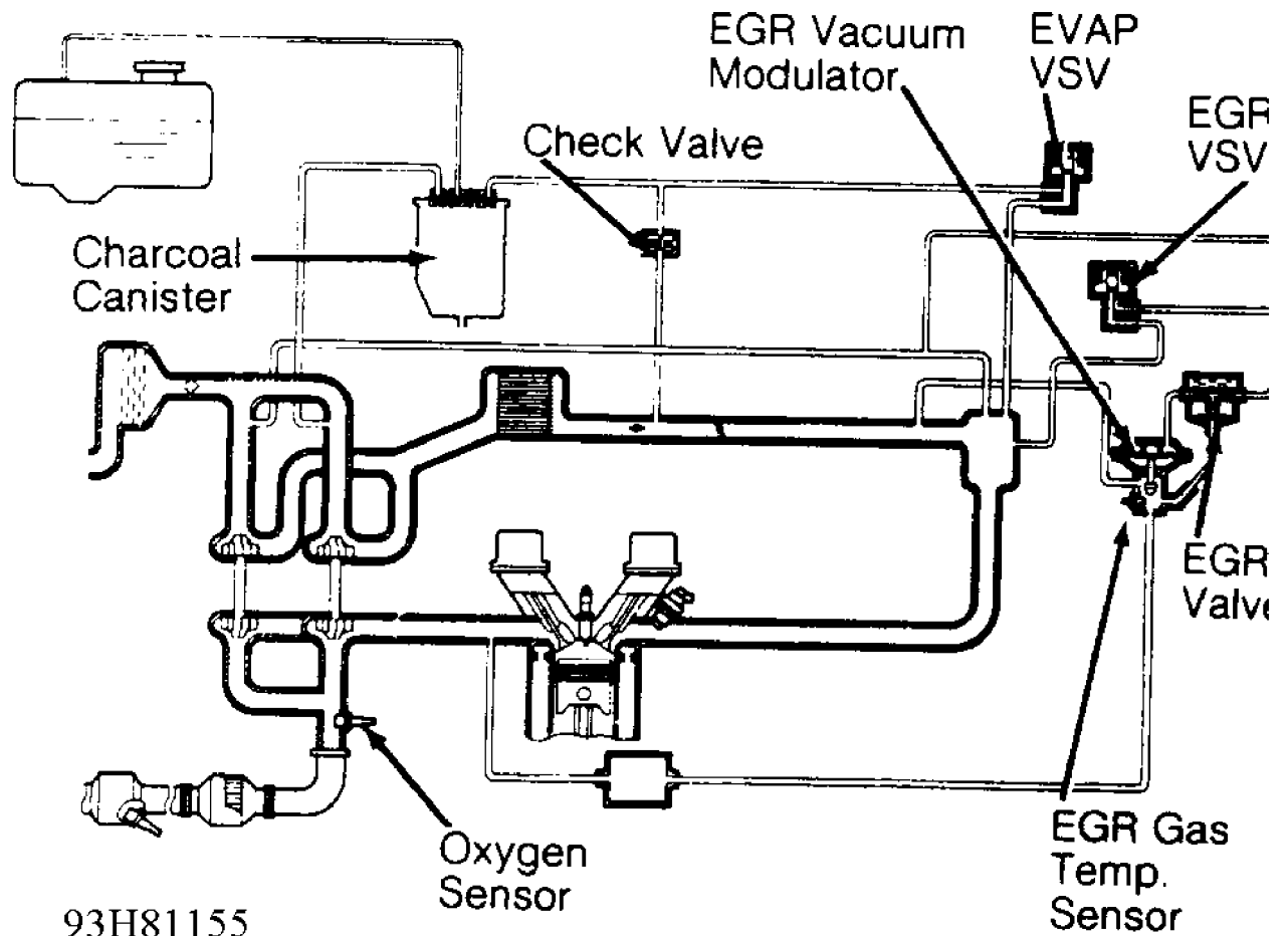
Fig. 25: Vacuum Diagram (Supra Turbo)
