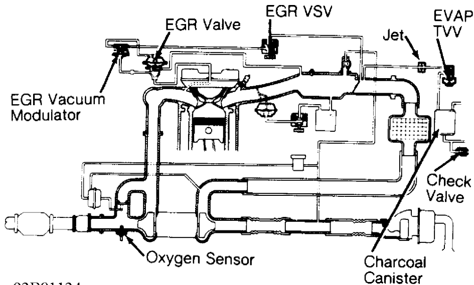
Fig. 5: Vacuum Diagram (Celica 2.0L Turbo 3S-GTE - Schematic) Courtesy of Toyota Motor Sales, U.S.A., Inc.
