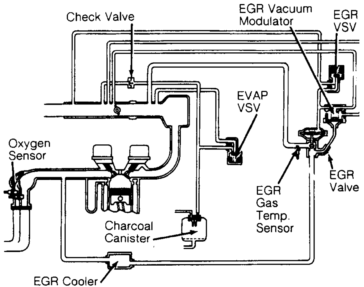
M-VACUUM 93F81153 Fig. 23: Vacuum Diagram (Supra Non-Turbo - Schematic) Courtesy of Toyota Motor Sales, U.S.A., Inc.
