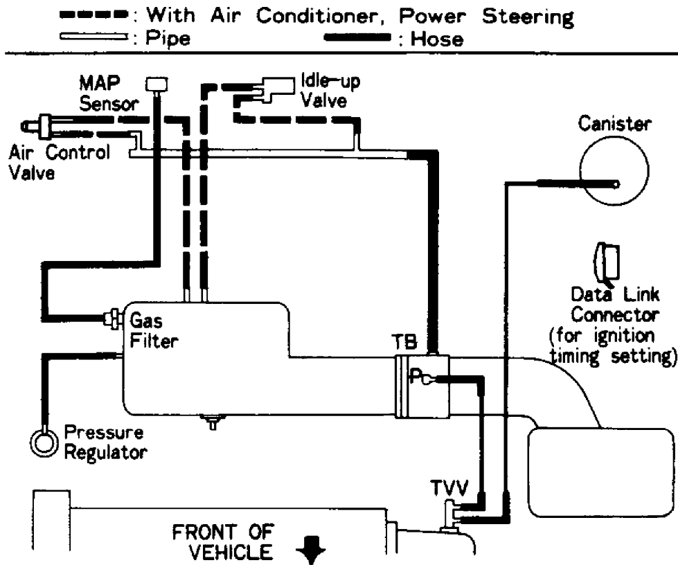
93D81136 Fig. 7: Vacuum Diagram (Corolla - Federal Models) Courtesy of Toyota Motor Sales, U.S.A., Inc.
