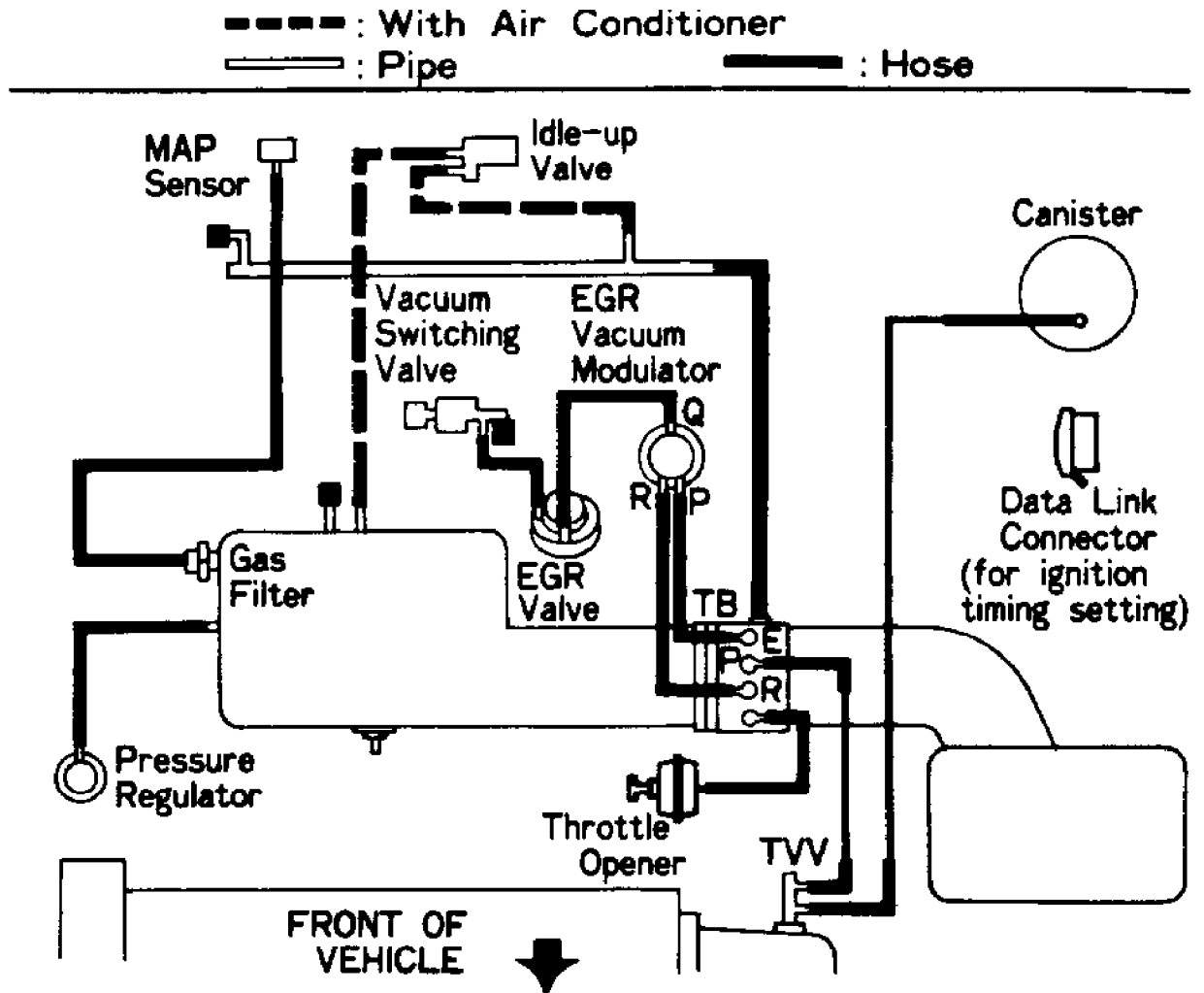
Fig. 9: Vacuum Diagram (Corolla - Calif. Models W/O Power Steering)
