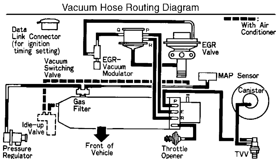
Fig. 1: Vacuum Diagram (Camry 2.2L)
