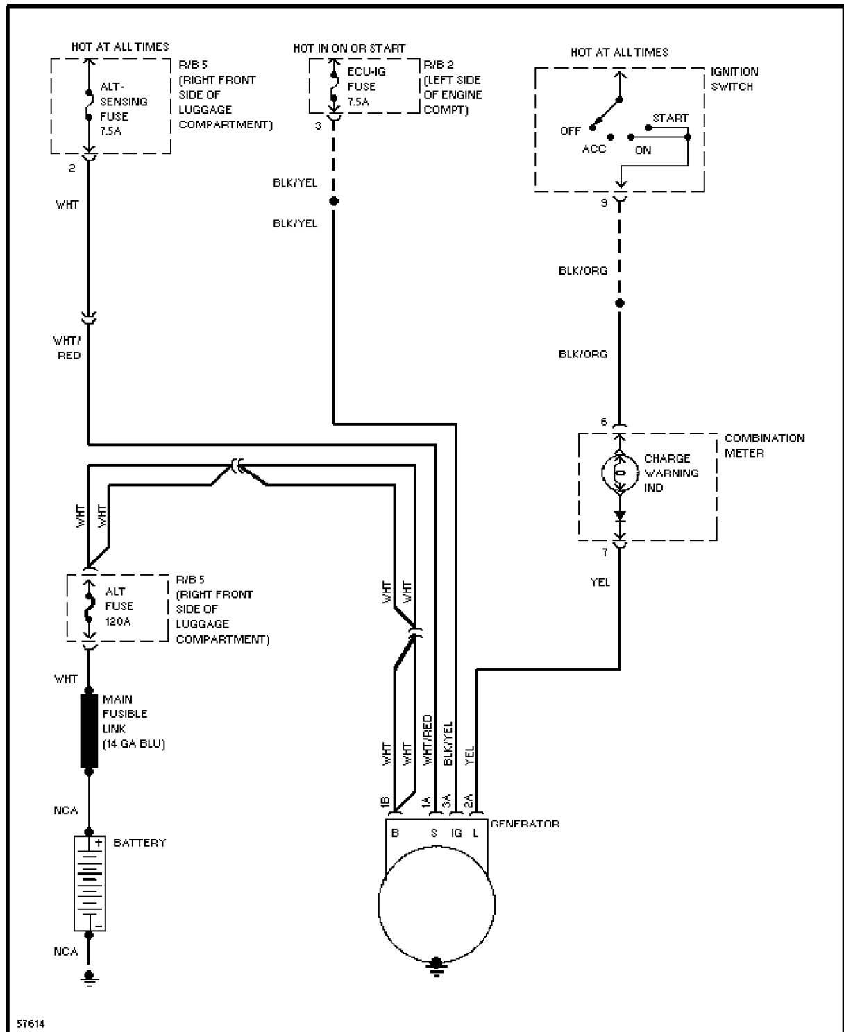
Charging Circuit
