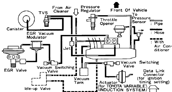
Fig. 2: Vacuum Diagram (Turbo)
