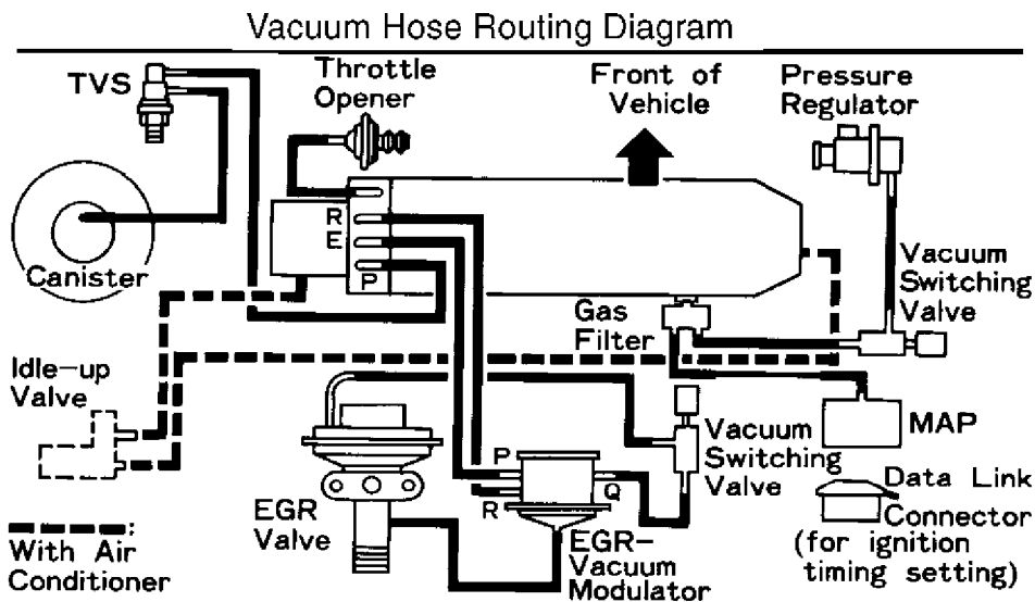
Fig. 1: Vacuum Diagram (Non-Turbo)
