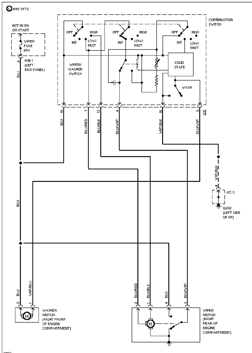
Wiper/Washer Circuit
