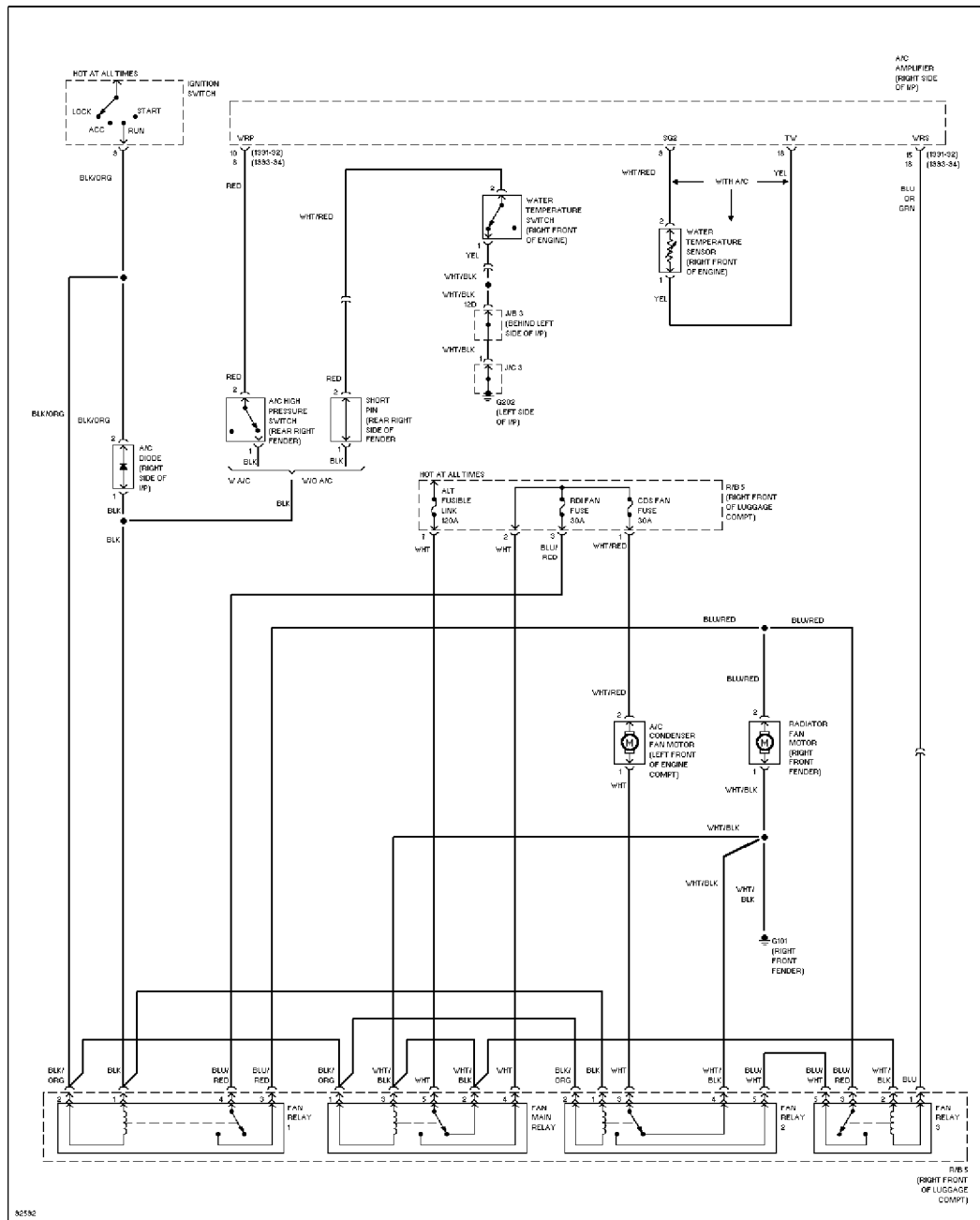
Radiator Cooling Fan Circuit
