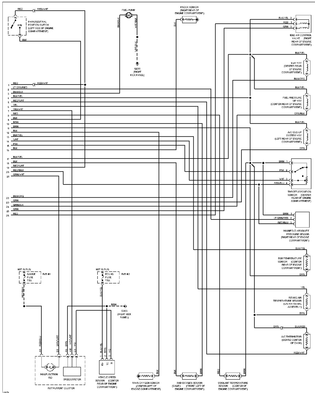
2.2L, Engine Performance Circuits, A/T (2 of 2) SYSTEM WIRING DIAGRAMS Article Text (p. 17)1994 Toyota MR2For Rse 555 Main Street Clarksville Va 229
