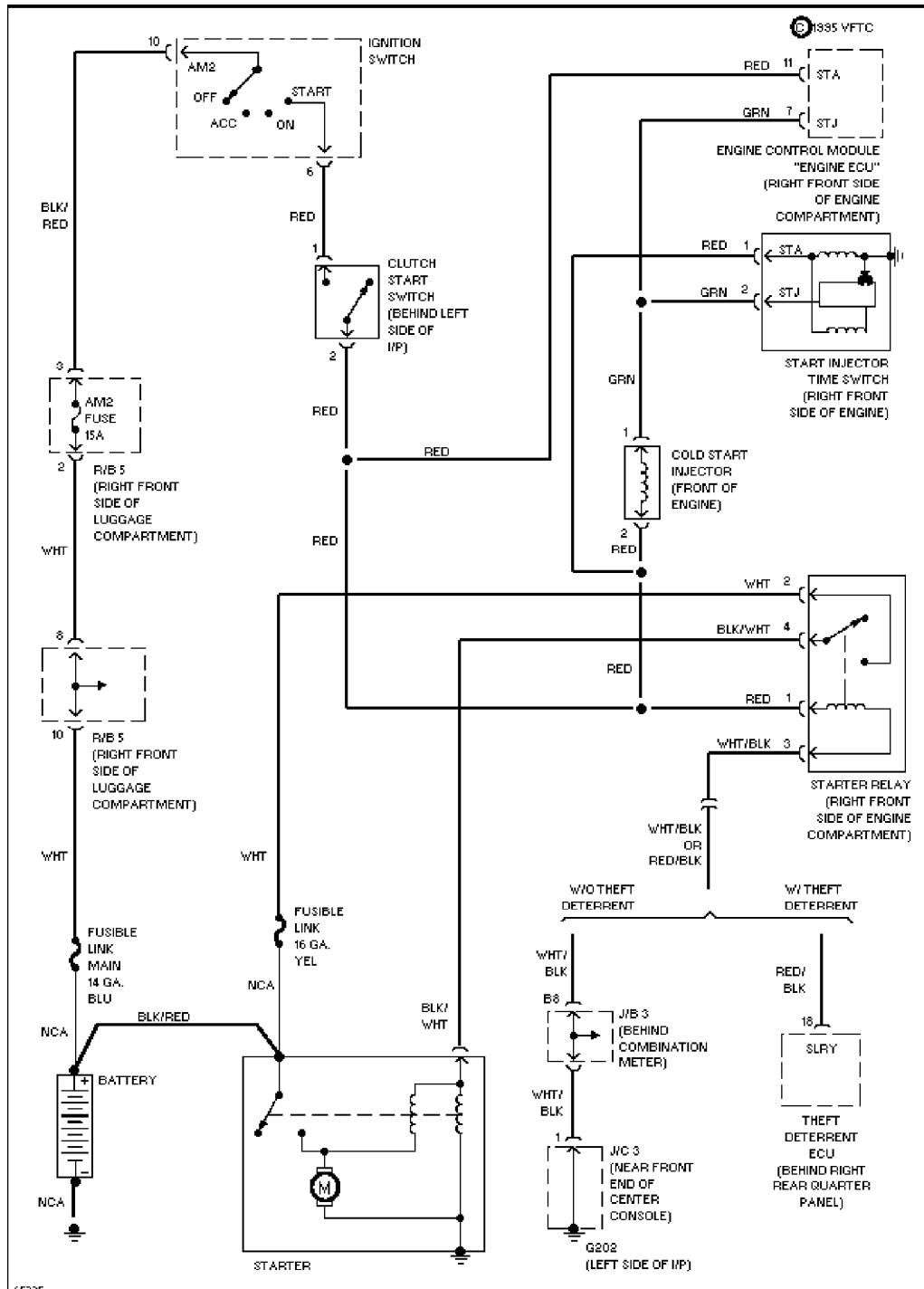
2.0L Turbo, Starting Circuit
