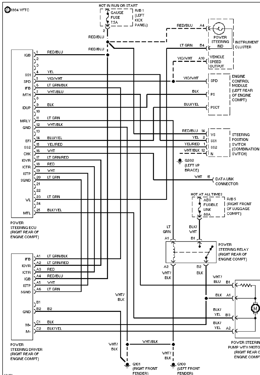
Electronic Power Steering Circuit
