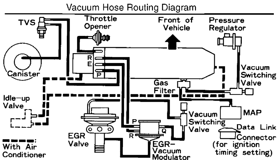
Fig. 1: Vacuum Diagram
