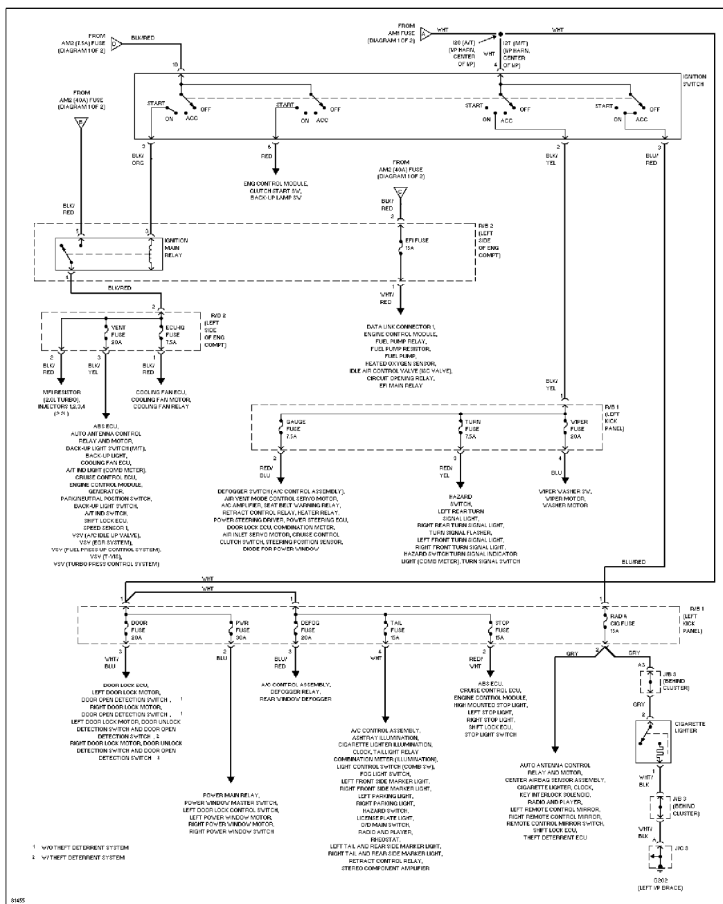
Power Distribution Circuit (2 of 2)
