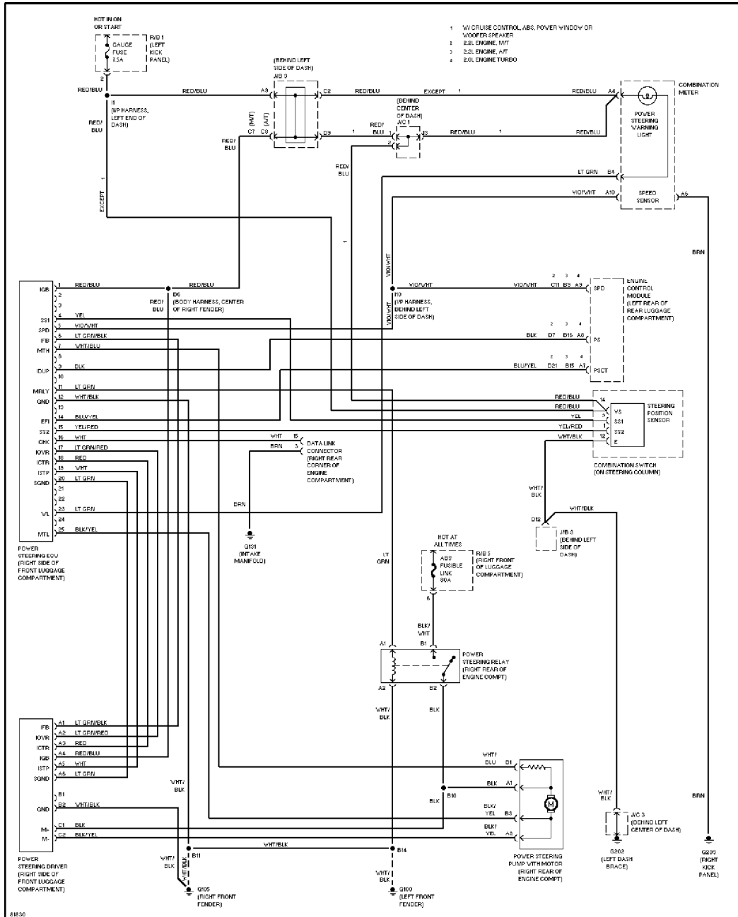
Electronic Power Steering Circuit
