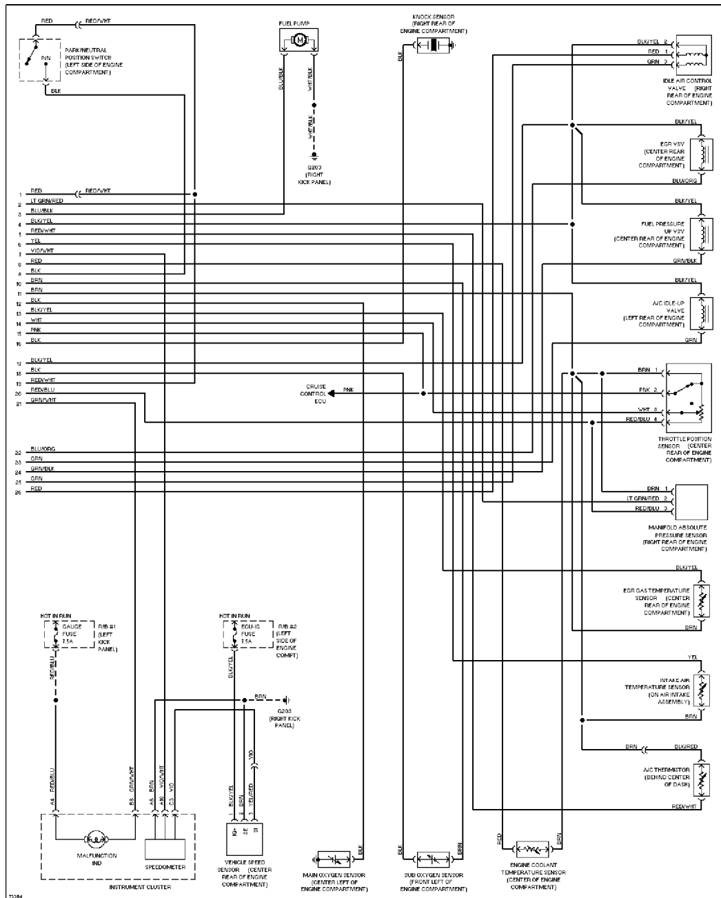
2.2L, Engine Performance Circuits, A/T (2 of 2) SYSTEM WIRING DIAGRAMS Article Text (p. 14)1995 Toyota MR2For Rse 555 Main Street Clarksville Va 229
