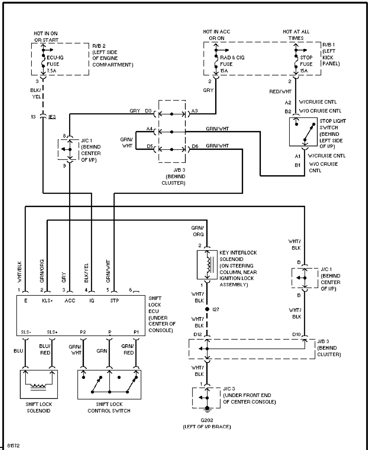
SYSTEM WIRING Shift Interlock Circuit
